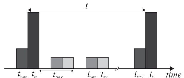
FIGURE 6. Model for the transceiver to be powered by RF energy harvester [47].
