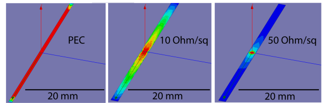
FIGURE 3. The surface currents on dipole antenna elements with the colored scale are the same in all three cases (from left to right) for a perfect electrical conductor (PEC), R_{sh} = 10 \Omega/sq and R_{sh} = 50 \Omega/sq , respectively.
