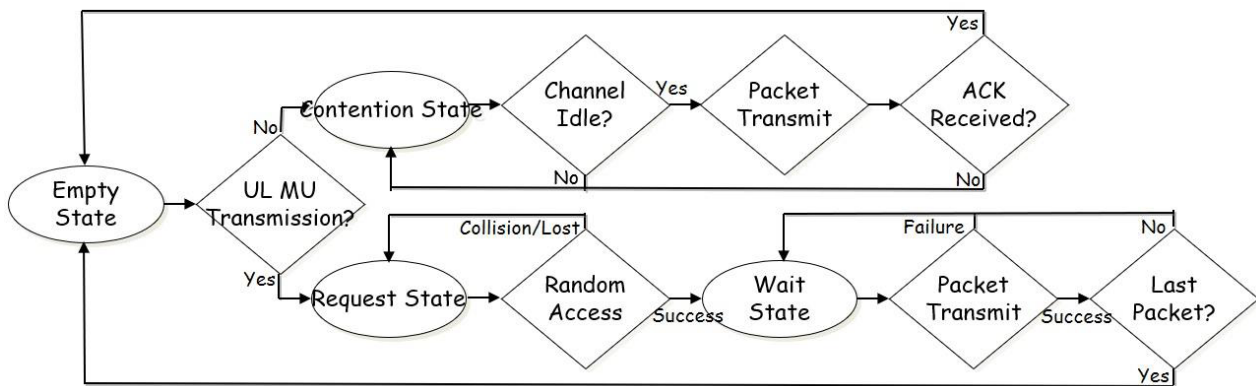
FIGURE 13. HE STA's state transition diagram.
