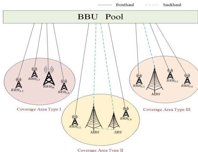
FIGURE 4. Flexible constructions for the network architecture of H-CRANs.
