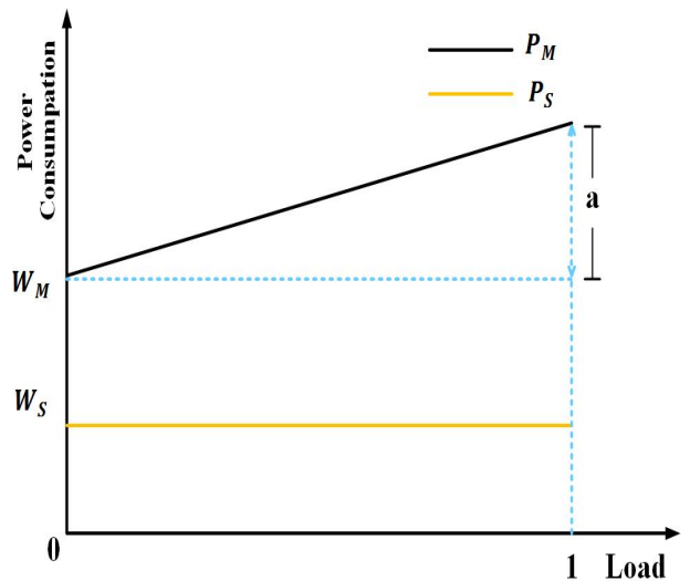
FIGURE 1. Power consumption of MBS (denoted as P_M ) and Power consumption of SBS (denoted as P_S ) as a function of the traffic load [20]. ( P_M = a \times \text{load} + W_M where a is linear coefficient and W_M is the basic circuit power consumption of a MBS when there is no traffic load, P_S = W_S where W_S is a constant independent of traffic load.)
