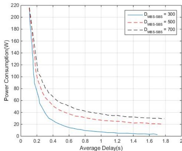
FIGURE 2. Energy-delay tradeoff for different densities of SBS deployment (denoted by average distances between the MBS and SBSs, D_{\text{MBS-SBS}} ) when the average traffic load of SBSs is given as \rho = 0.30 , where \rho = \lambda/\mu with \lambda being the total arrive rate of flows and \mu being the serving rate in the modeled Markov process [27].
