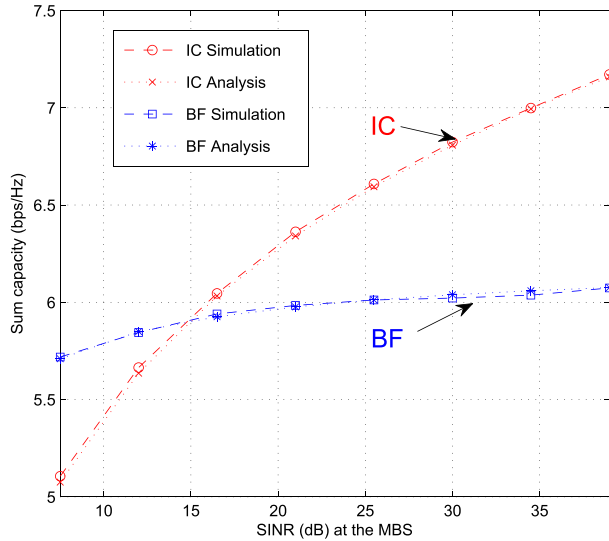
FIGURE 4. System sum capacity under IC and BF schemes versus the SINR (dB) at the MBS for H-CRANs.
