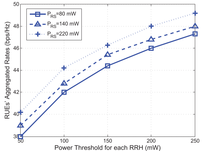
FIGURE 7. RUEs' aggregated rates under the BF scheme versus the power threshold (mW) for H-CRANs.
