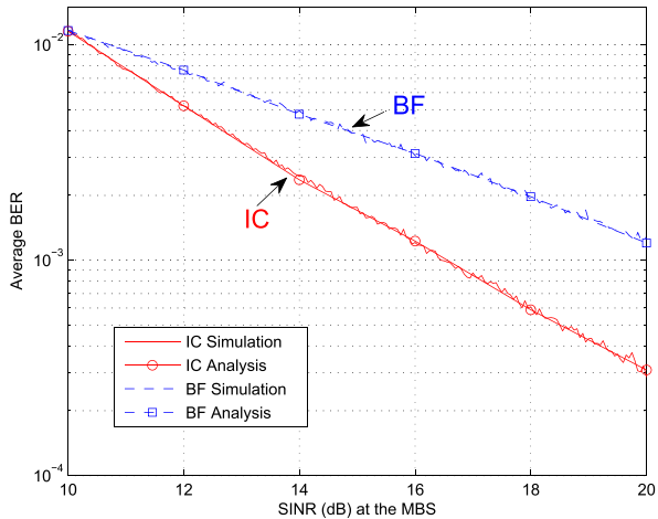
FIGURE 5. Average BER under IC and BF schemes versus the SINR (dB) at the MBS for H-CRANs.
