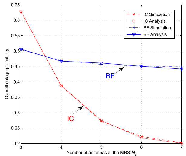
FIGURE 3. Overall outage probability versus the number of antennas N_B .
