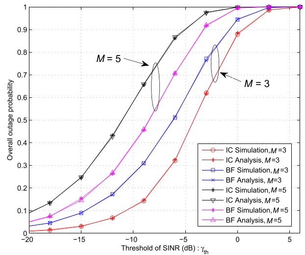
FIGURE 2. Overall outage probability under IC and BF schemes.
