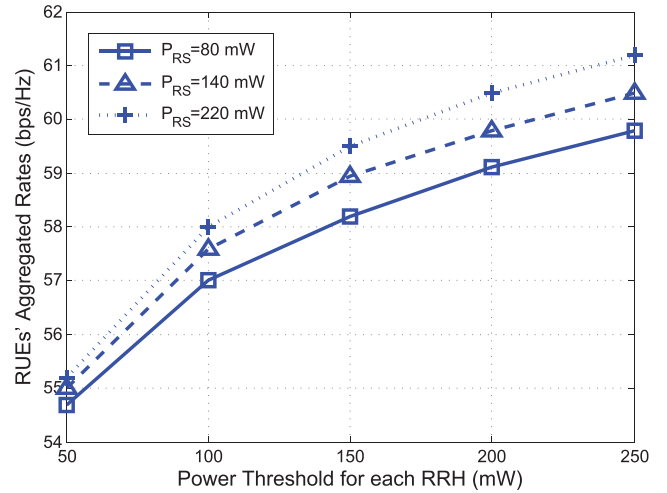
FIGURE 6. RUEs' aggregated rates under the IC scheme versus the power threshold (mW) for H-CRANs.
