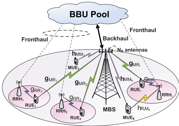
FIGURE 1. System model of an H-CRAN with one MBS and M RRHs.
