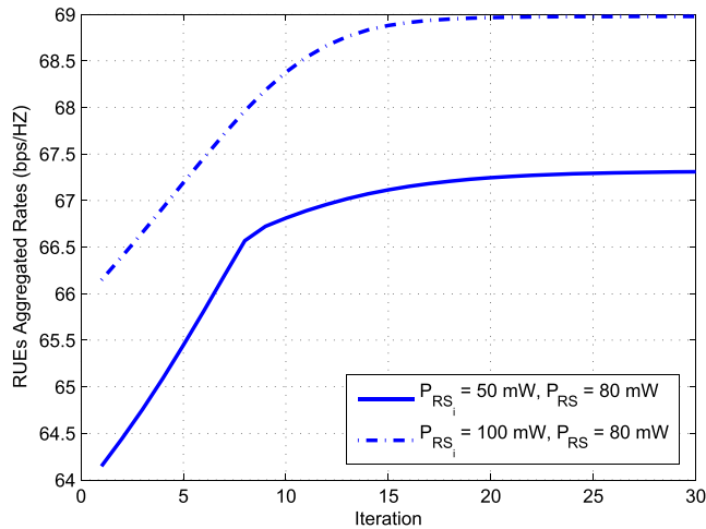
FIGURE 8. Convergence behavior of the RUEs' aggregated rates under the IC scheme.
