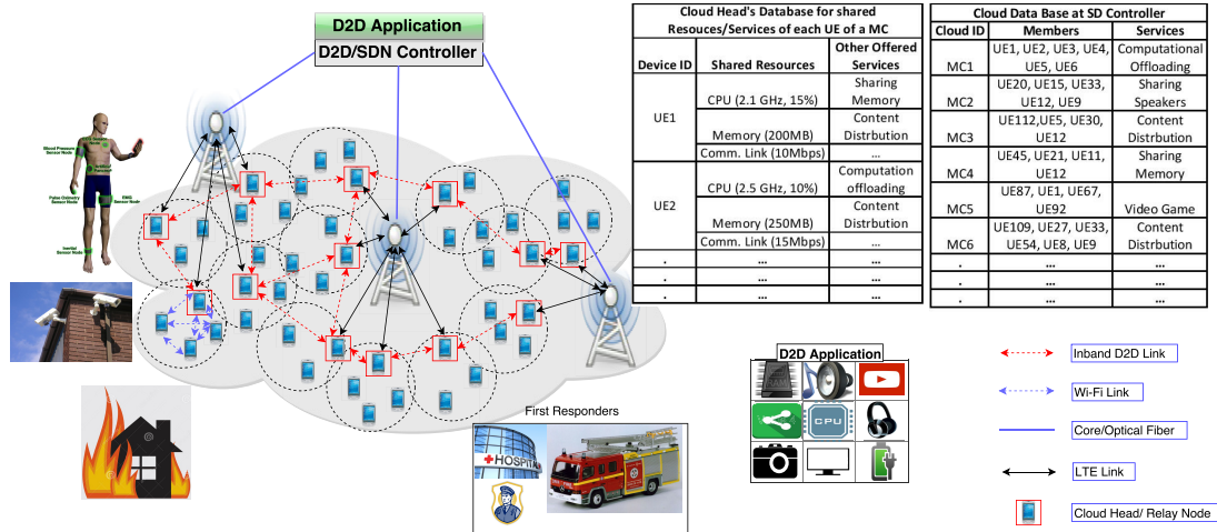
FIGURE 1. The proposed Software-Defined D2D communication architecture for public safety applications.
