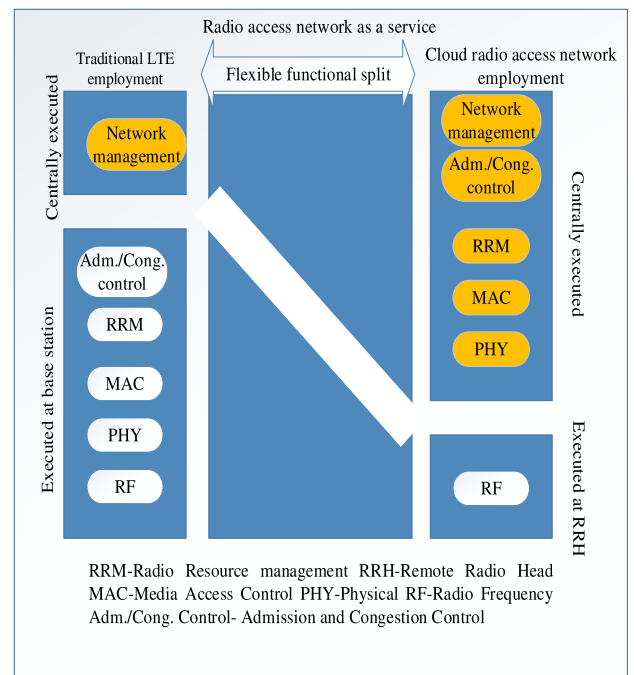
FIGURE 12. Flexible functional split [103].
