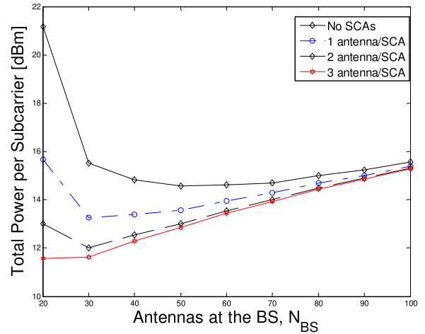
FIGURE 4. Average total power consumption in the scenario containing small cell access points.
