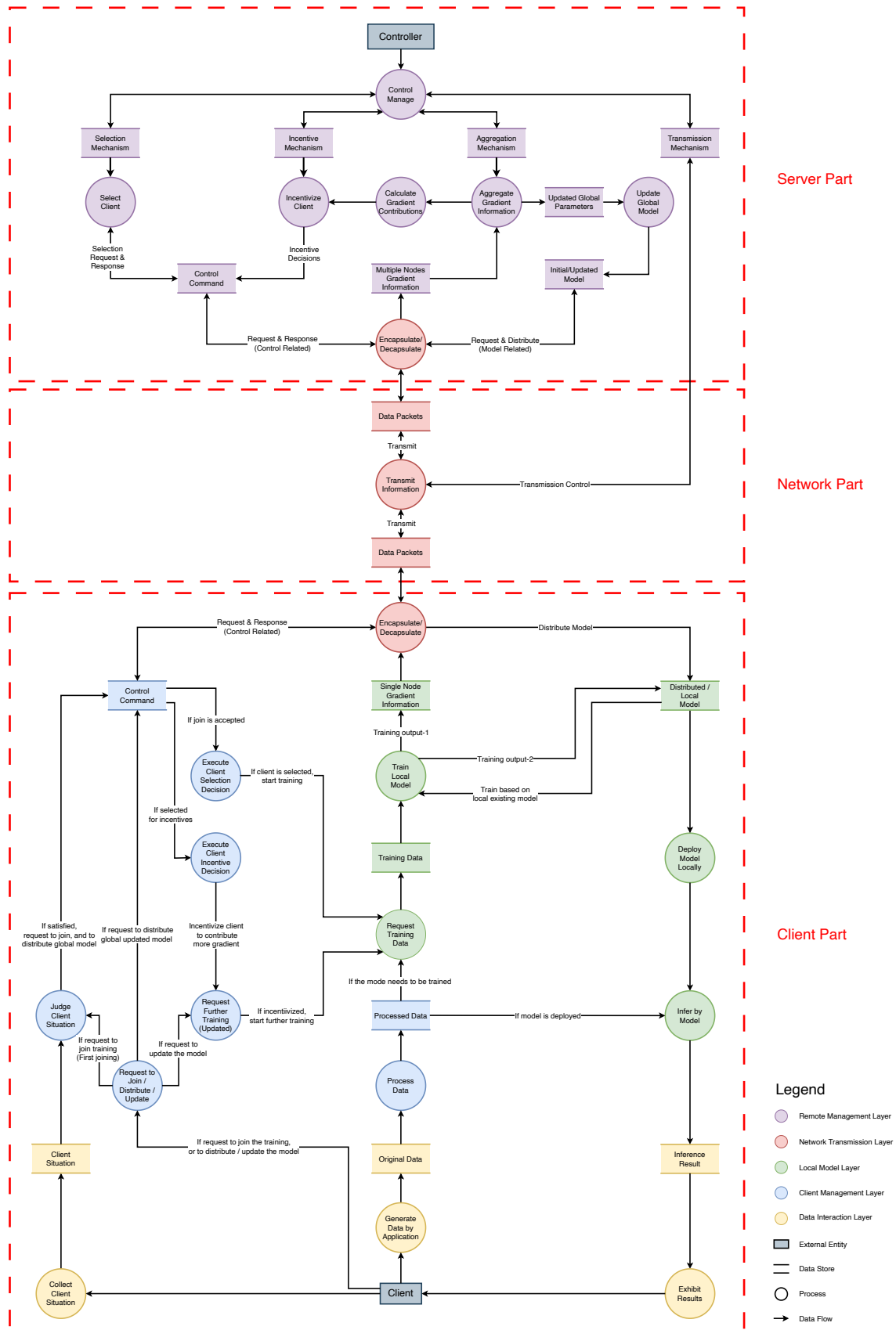
FIGURE 4. Low-level Data Flow of Federated Learning
