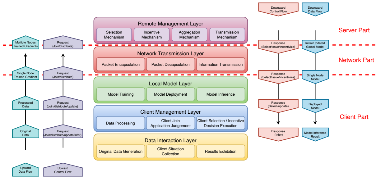
FIGURE 3. Proposal of 5-layer Federated Learning Reference Model
