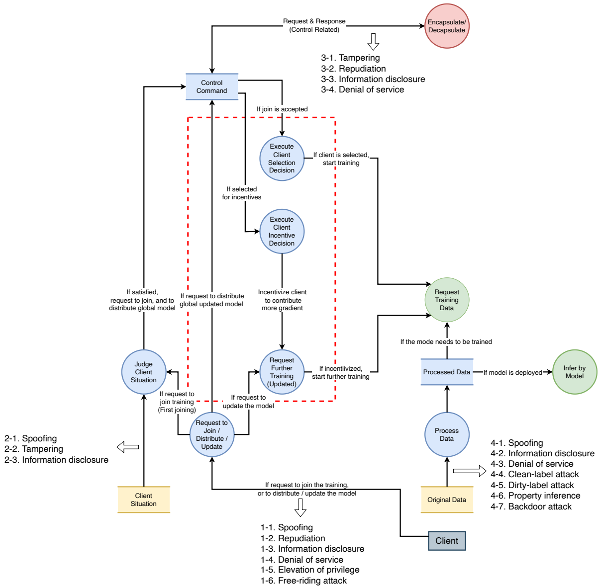
FIGURE 7. Threats in Client Management Layer
