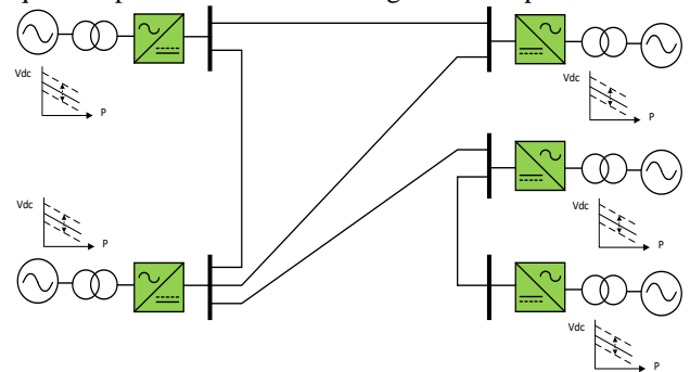
FIGURE 11. Generic model of centralized control
