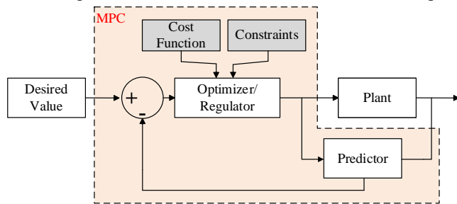
FIGURE 13. MPC control structure [83]
