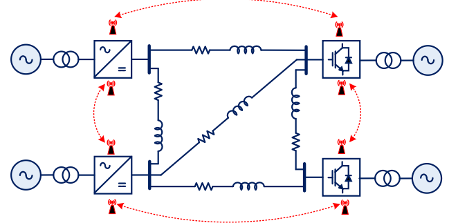
FIGURE 12. Generic model of distributed control
