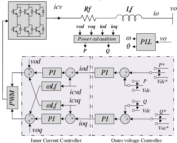
FIGURE 8. Structure of primary control layers [33]
