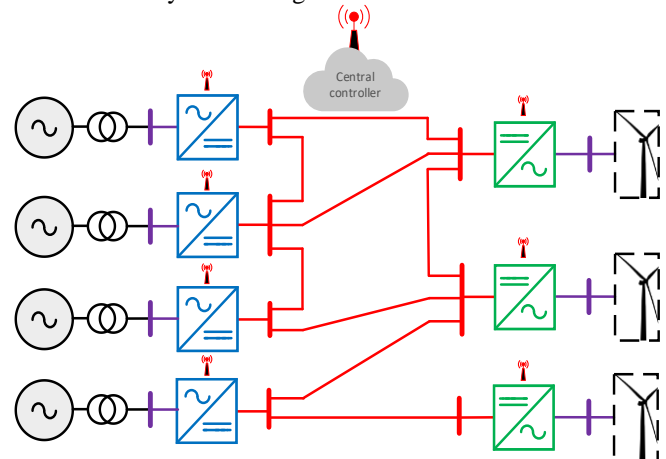
FIGURE 10. Generic model of centralized control
