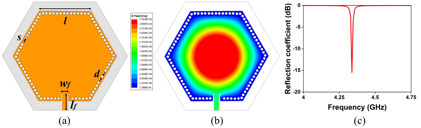
FIGURE 1. Geometry of the single port hexagonal SIW antenna [ l = 19.5 , s = 1.4 , d = 1 , l_f = 6.69 , w_f = 2 (all are in mm)]
