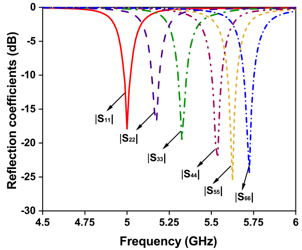
FIGURE 3. Reflection coefficient plot of the proposed self-hexaplexing antenna.
