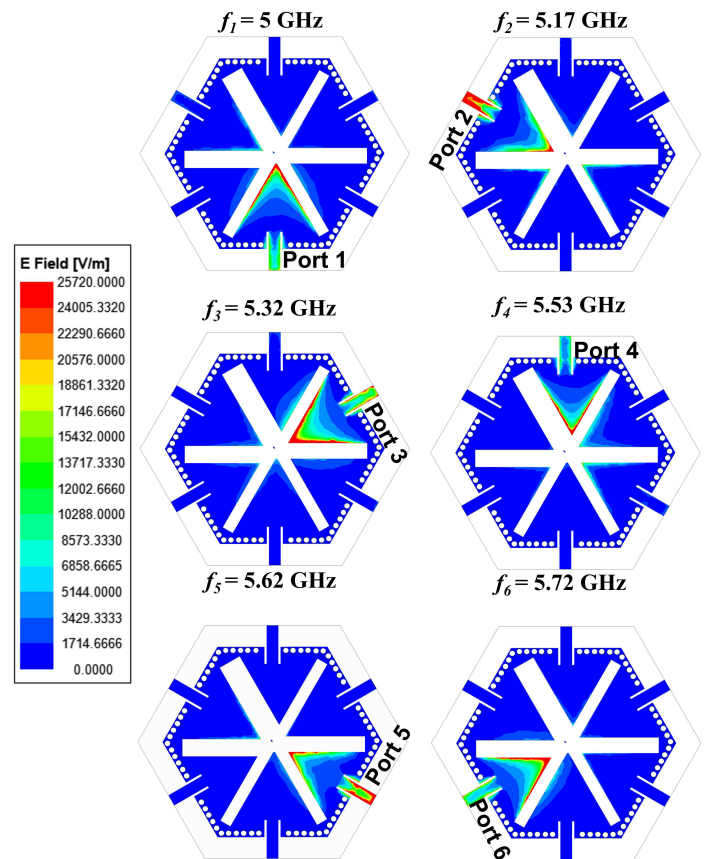
FIGURE 7. Electric field distribution at six resonating frequencies.
