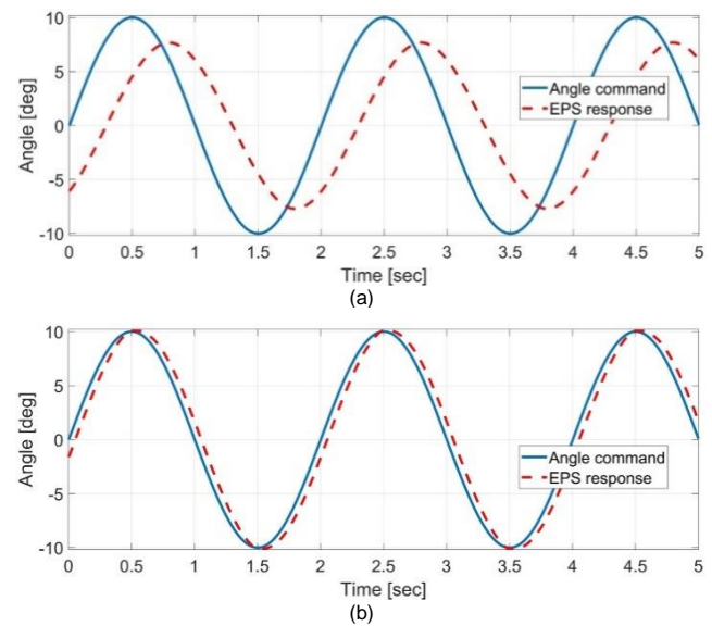
FIGURE 4. Output responses by PID parameter tuning: (a) EPS response with a lower constant of K_1=0.04 , K_2=0.0095 , and K_3=0.0000025 , (b) EPS response with optimal constants of K_1=0.113 , K_2=2.016 , and K_3=0.0000025 .
