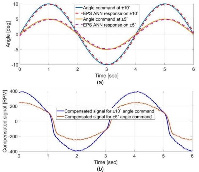
FIGURE 14. Time response results of EPS using ANN controller with sine wave input at a frequency of 0.25 Hz: (a) Responses on EPS angle target of \pm 10^\circ and \pm 5^\circ , (b) The compensated signals.
