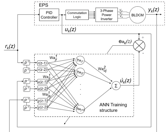
FIGURE 8. Proposed ANN Controller Training Model for EPS
