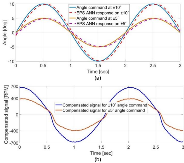
FIGURE 15. Time response results of EPS using ANN controller with sine wave input at a frequency of 0.5 Hz: (a) Responses on EPS angle target of \pm 10^\circ and \pm 5^\circ , (b) The compensated signals.
