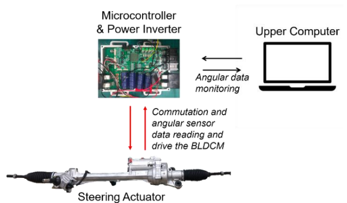
FIGURE 10. EPS testbed setup for Proposed ANN controller reviews.
