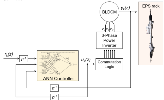
FIGURE 9. Overall EPS block diagram with Proposed ANN controller
