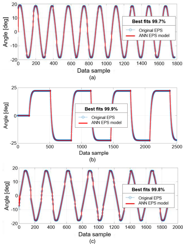
FIGURE 12. The time response outcomes for both the original EPS and the identified ANN model with network topology of 5-5-1, 100 learning iterations, and LR=0.1. The responses to: (a) Sine wave, (b) Square wave, (c) Triangular wave.
