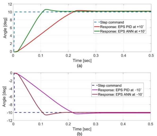
FIGURE 17. EPS response results on step input of \pm 10^\circ : (a) EPS response using PID and ANN controllers in clockwise rotation, (b) EPS response using PID and ANN controllers in counterclockwise rotation.
