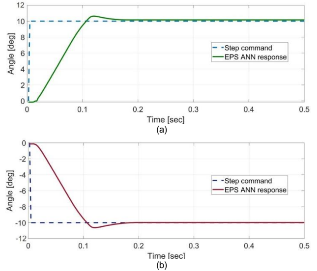
FIGURE 13. EPS response on step input of \pm 10^\circ : (a) EPS response using ANN controller in clockwise rotation, (b) EPS response using ANN controller in counterclockwise rotation.
