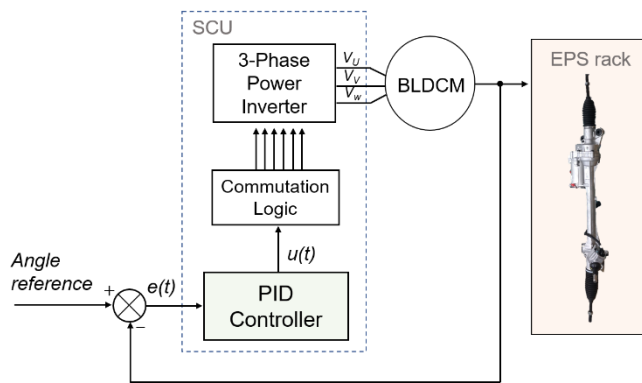
FIGURE 3. EPS scheme of SCU with PID controller.
