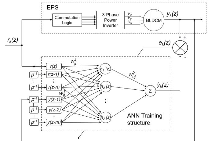
FIGURE 7. Proposed ANN structure for EPS identification.
