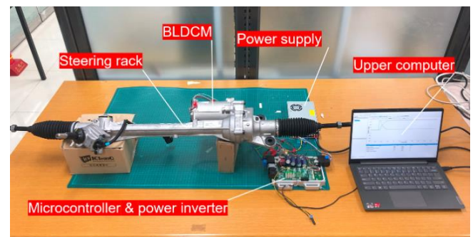
FIGURE 5. Experimental setup.
