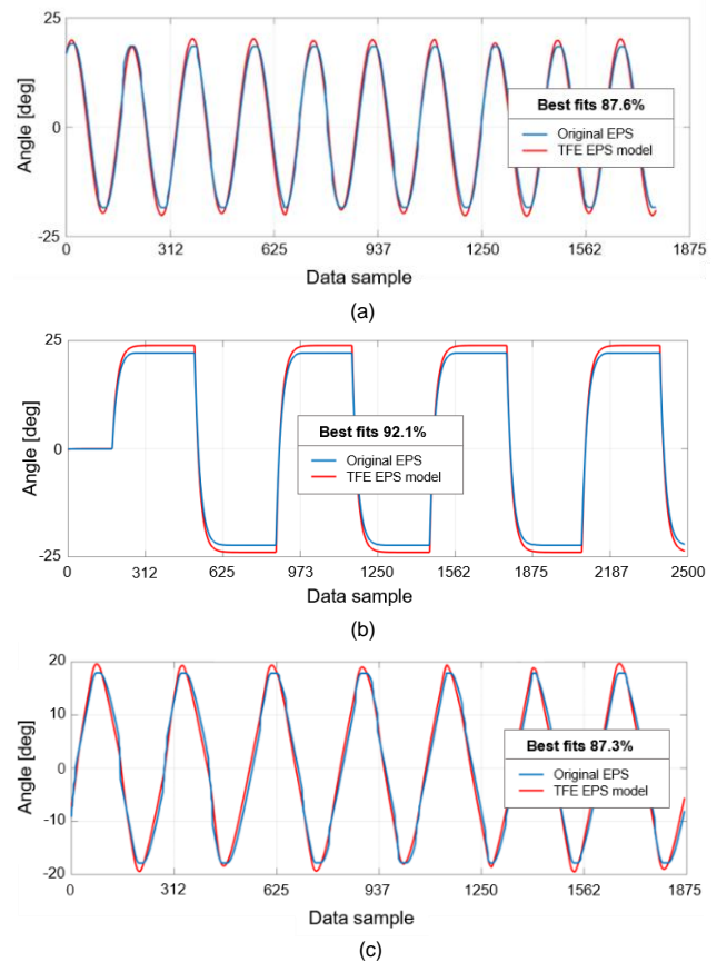
FIGURE 11. The time response outcomes for original EPS and the simplified 2 nd order TFE model (a) Response to the sine wave, (b) Response to the square wave, (c) Response to the triangular wave.
