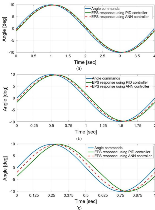
FIGURE 18. EPS PID and EPS ANN controllers output performance comparison corresponding to the provided input sine wave with angle target peak to peak of \pm 10^\circ : (a) At a frequency of 0.25 Hz, (b) At a frequency of 0.5 Hz, (c) At a frequency of 1 Hz.
