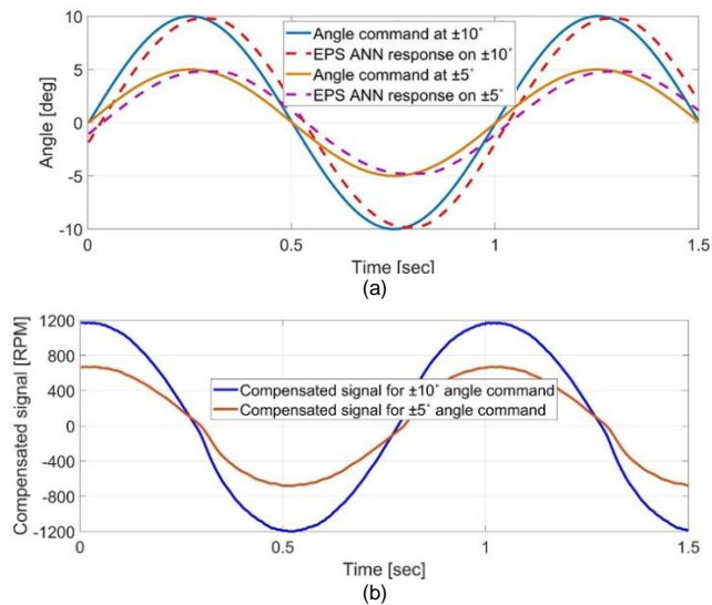
FIGURE 16. Time response results of EPS using ANN controller with sine wave input at a frequency of 1 Hz: (a) Responses on EPS angle target of \pm 10^\circ and \pm 5^\circ , (b) The compensated signals.
