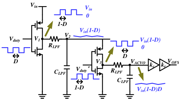
FIGURE 18. Implementation of Auto-Correction of Voltage Offset (ACVO)
