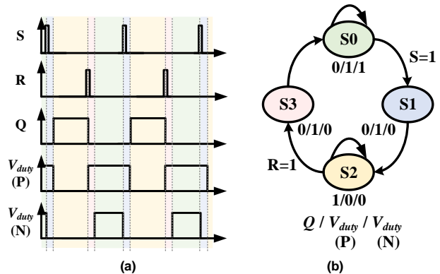
FIGURE 8. SR-latch (a) waveform diagram (b) state machine
