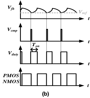
FIGURE 2. An example of the constant-on time control (a) circuit diagram (b) control waveforms
