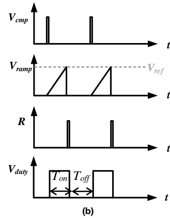
FIGURE 3. Commonly used constant on timer (a) circuit diagram (b) waveform
