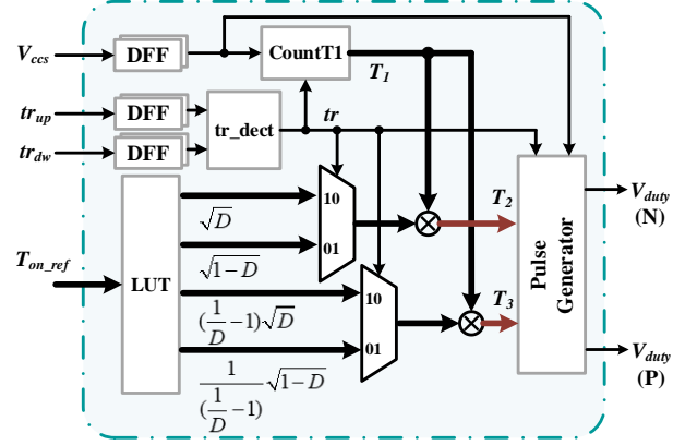
FIGURE 11. The block diagram of the digital transient-optimized control (DTOC)
