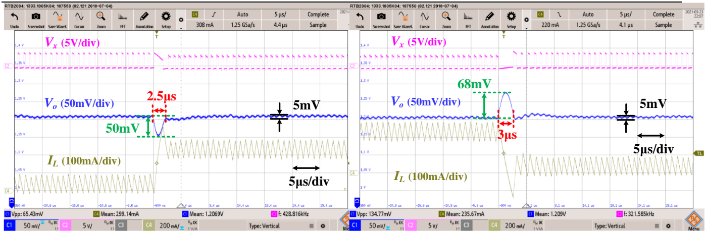
(c) light to heavy load with DTOC (d) heavy to light load with DTOC
