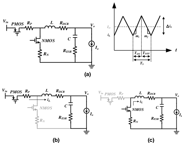
FIGURE 4. Non-ideal power stage of a buck converter (a)circuit and its waveform (b) The upper arm (PMOS) is conducting (c) The lower arm (NMOS) is conducting
