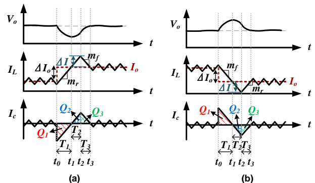
FIGURE 10. Load transient timing diagram (a) load step-up response (b) load step-down response
