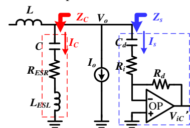
FIGURE 17. Implementation of the CCS
