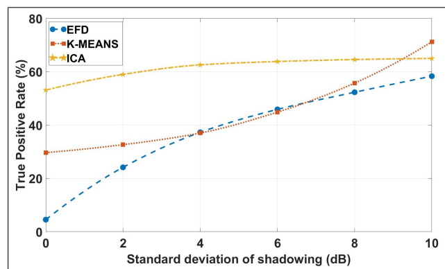
FIGURE 10: True positive rate of small cell outage detection over varying shadowing with EFD, k-means clustering and ICA
