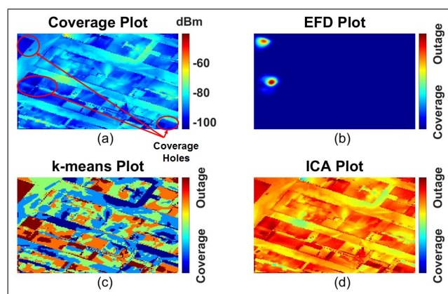
FIGURE 4: Coverage hole detection using EFD, k-means clustering and ICA with 0 dB open space shadowing
