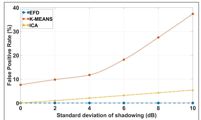
FIGURE 15: False positive rate of mmWave cell outage detection over varying shadowing with EFD, k-means clustering and ICA
