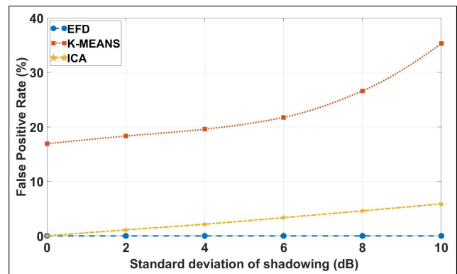
FIGURE 11: False positive rate of small cell outage detection over varying shadowing with EFD, k-means clustering and ICA
