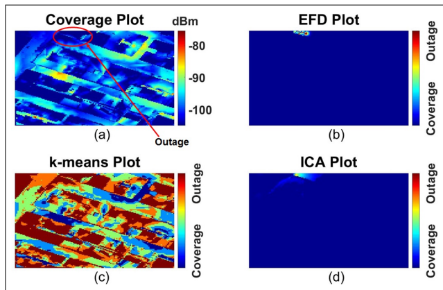
FIGURE 13: mmWave cell outage detection using EFD, k-means clustering and ICA with 10 dB open space shadowing show the results of k-means clustering, while Subfigs. (d) show the results for ICA algorithm.
