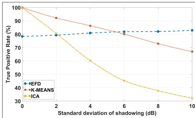
FIGURE 6: True positive rate of coverage hole detection over varying shadowing with EFD, k-means clustering and ICA
