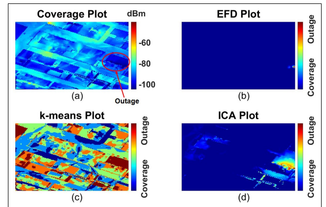
FIGURE 8: Small cell outage detection using EFD, k-means clustering and ICA with 0 dB open space shadowing
