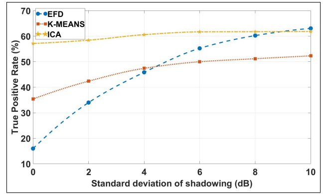
FIGURE 14: True positive rate of mmWave cell outage detection over varying shadowing with EFD, k-means clustering and ICA
