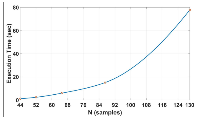
FIGURE 1: Complexity of EFD-based outage and coverage hole detection algorithm
