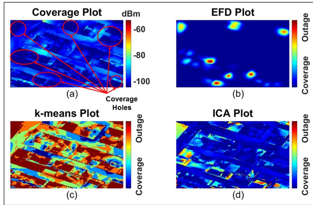
FIGURE 5: Coverage hole detection using EFD, k-means clustering and ICA with 10 dB open space shadowing
