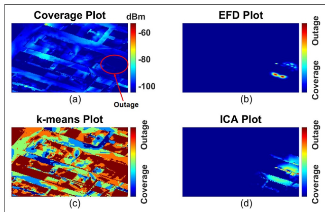
FIGURE 9: Small cell outage detection using EFD, k-means clustering and ICA with 10 dB open space shadowing
