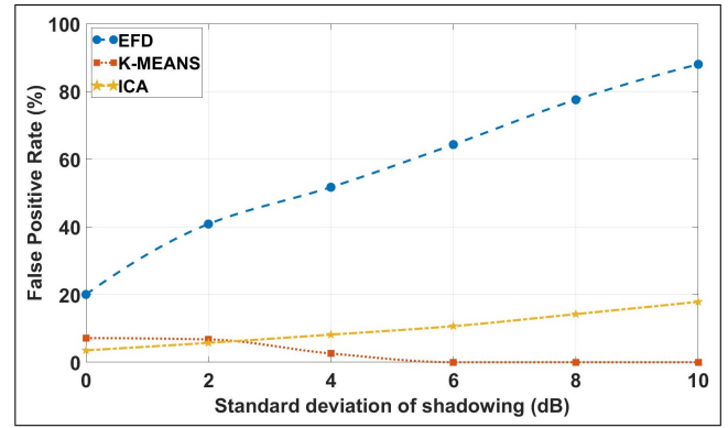
FIGURE 7: False positive rate of coverage hole detection over varying shadowing with EFD, k-means clustering and ICA
