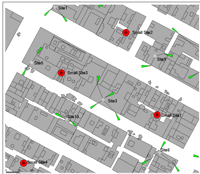
FIGURE 2: Network layout showing sites deployment.
