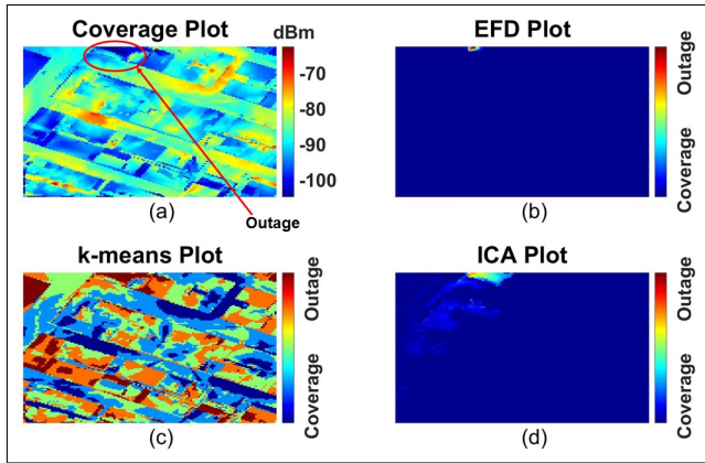
FIGURE 12: mmWave cell outage detection using EFD, k-means clustering and ICA with 0 dB open space shadowing
