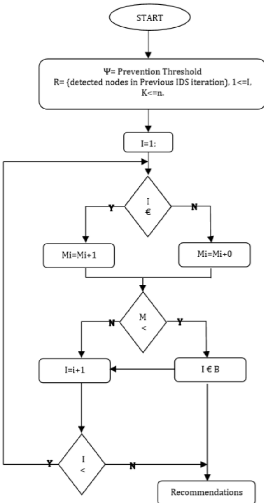
Fig. 2: Proposed IPAM algorithm flowchart
