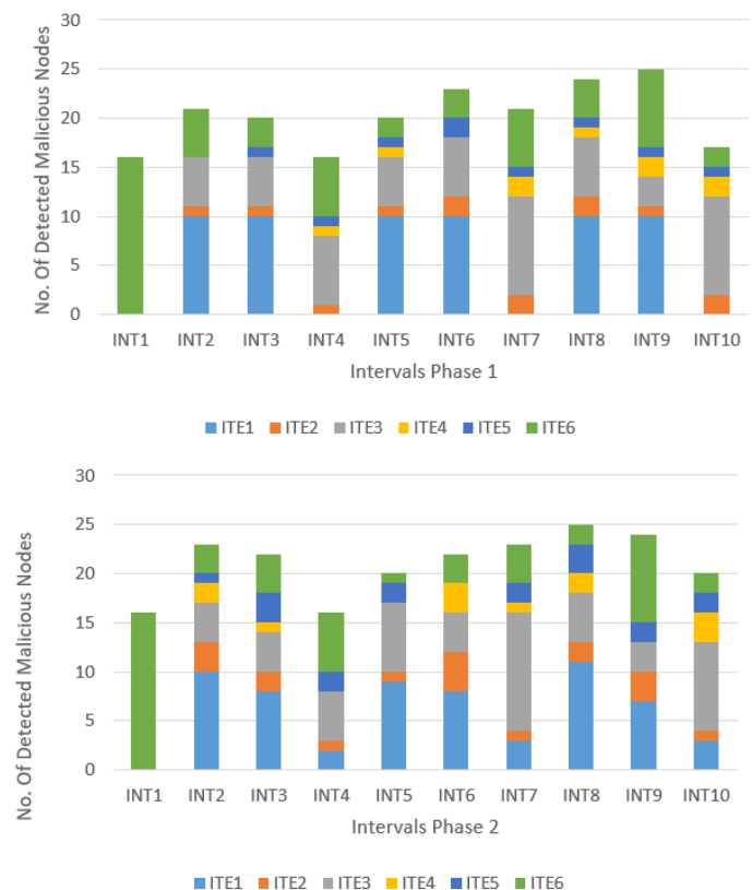
Figure 4. Detected malicious nodes in IoT with 10% Attackers.
