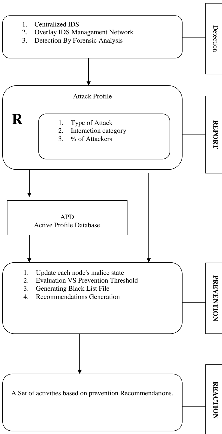
Figure 1: Proposed Security System Overview
