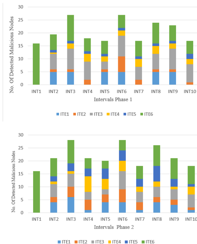
Figure 3. Detected malicious nodes in IoT with 5% Attackers.
