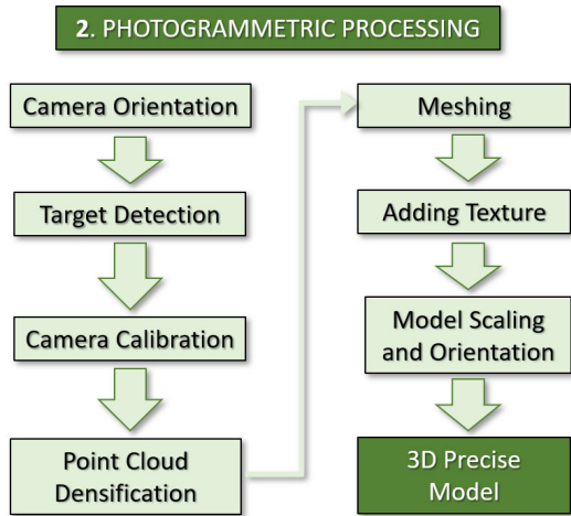
FIGURE 11. Photogrammetric processing flowchart.
