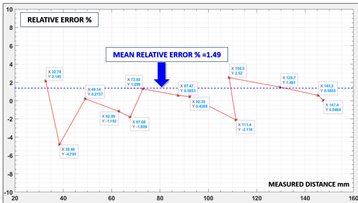
FIGURE 16. Relative error (%) vs. measured distance and mean relative error.
