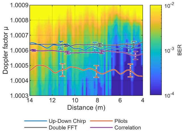
FIGURE 12. The value of the \mu coefficient as a function of the distance between the transmitter and receiver for different methods of determining the Doppler factor for a transmitter moving at 1 m/s.
