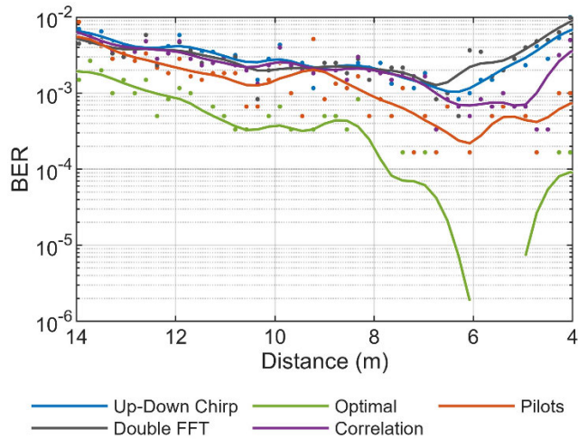
FIGURE 15. Data transmission quality as a function of the distance between the transmitter and receiver for different methods of determining the Doppler factor for a transmitter moving at 1.5 m/s.
