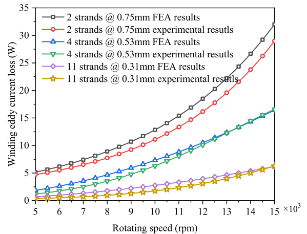
FIGURE 15. The 2D FEA and experimental test results of winding eddy current losses of Type I motors with three combinations of number and diameter of strands versus rotating speed.
