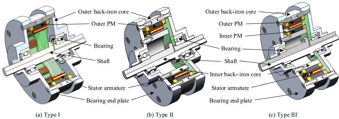
FIGURE 1. Analytical model of the three stator iron-core-less PMLDC motors. (a) Type I; (b) Type II; (c) Type III.
