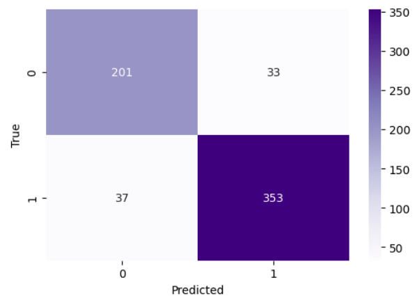
FIGURE 5. Confusion matrix for CNN model.
