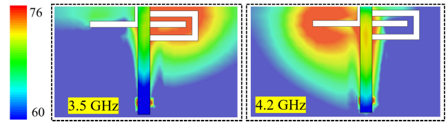
FIGURE 3. Surface current distribution at 3.5 and 4.2GHz.
