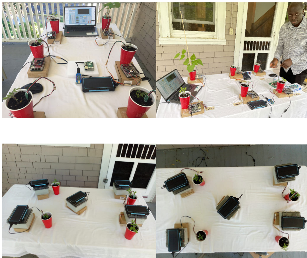
FIGURE 9. Proposed CA-IoT test-bed in full indoor operation mode.
