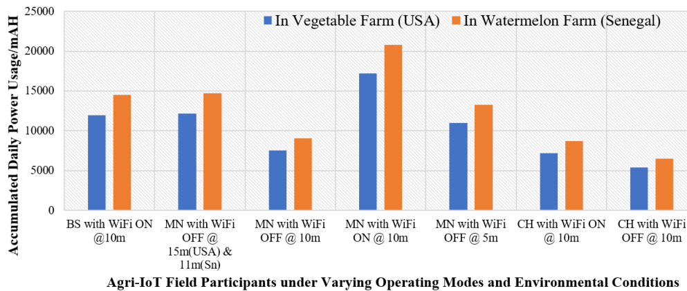
FIGURE 14. Comparing CA-IoT participants’ accumulated daily power consumptions at varying operating modes and d_{intra-c} under outdoor conditions.
