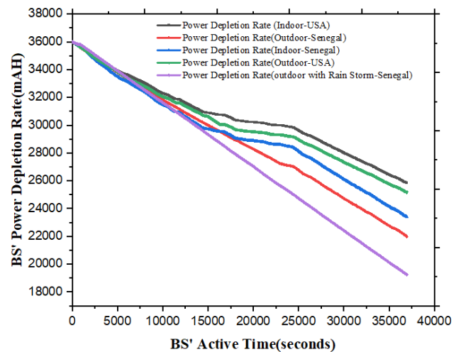
FIGURE 16. Sample BS' power depletion patterns under varying climatic conditions (at d_{intra-c} = 10m ).
