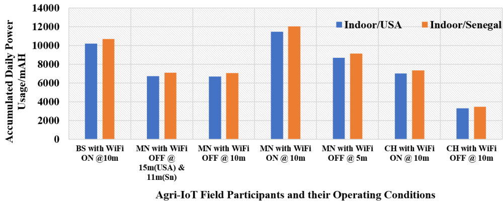
FIGURE 13. Comparing CA-IoT participants’ accumulated daily power consumptions at varying operating modes and d_{intra-c} under indoor conditions.
