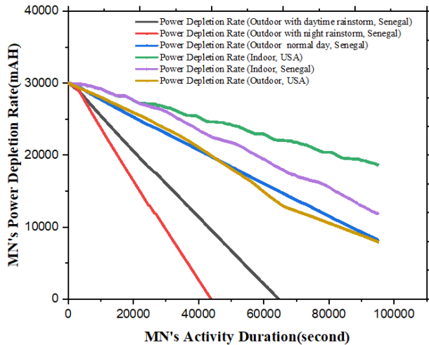
FIGURE 18. Sample MNs' power depletion patterns under varying climatic conditions (at d_{intra-c} = 10m ).
