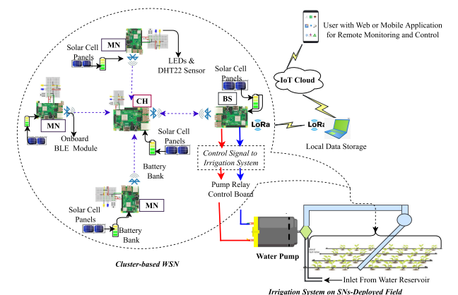
FIGURE 5. Custom-built WSN-based Agri-IoT architecture for precision irrigation application.
