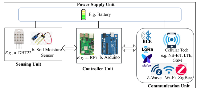
FIGURE 6. The principal components of SNs with sample design options in Agri-IoT.
