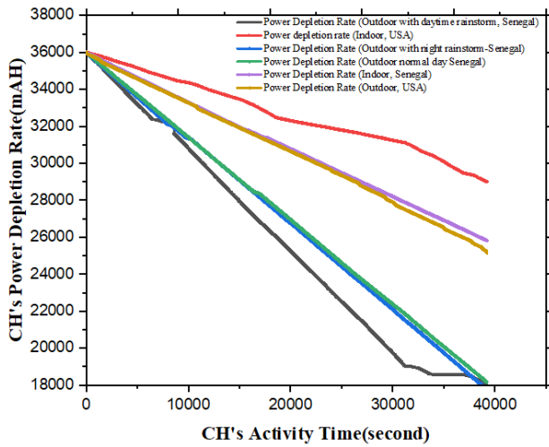
FIGURE 17. Sample CHs' power depletion patterns under varying climatic conditions (at d_{intra-c} = 10m ).
