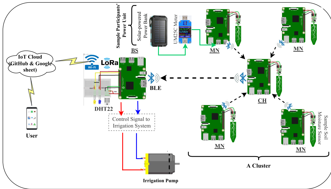
FIGURE 7. 1-Cluster schematic diagram of proposed CA-IoT implemented on test-bed.
