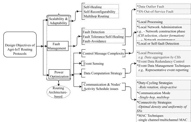
FIGURE 3. Expected design objectives of WSN-based Agri-IoT routing protocols with sample implementational strategies.
