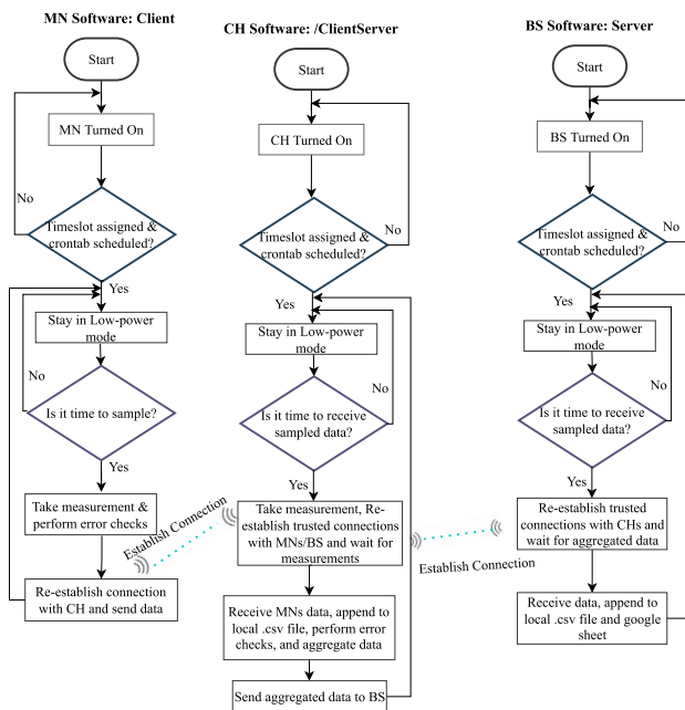
FIGURE 8. Flowcharts of the operational cycle of event routing software running on the MN, CH, and BS.
