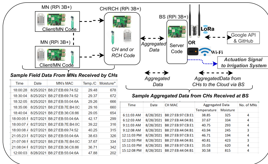
FIGURE 11. Data flow model of our CA-IoT network with sample measurements.
