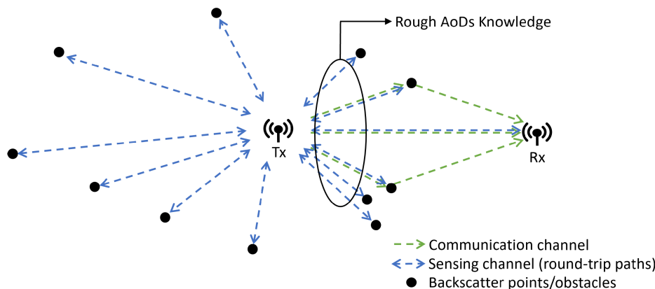
FIGURE 2. Sensing channel cluster geometry based on 3GPP GBSM, adjusted from [16], illustrates the correlation between communication and sensing channels.
