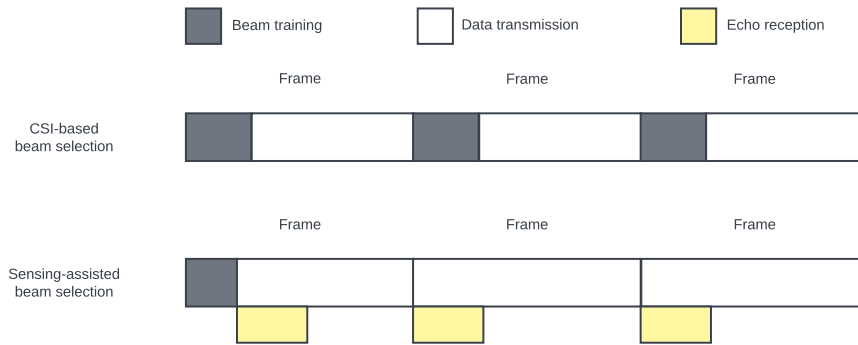
FIGURE 5. Frame structure in a DL transmission.
