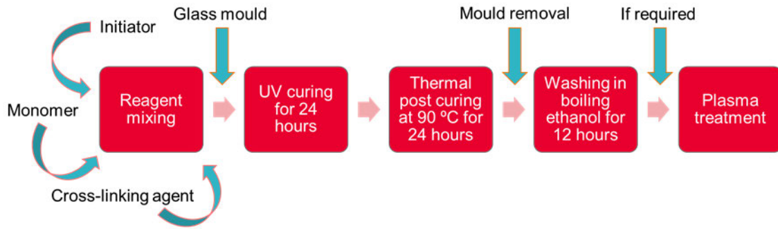
FIGURE 1. Manufacturing process of the different substrates for direct ink printing.
