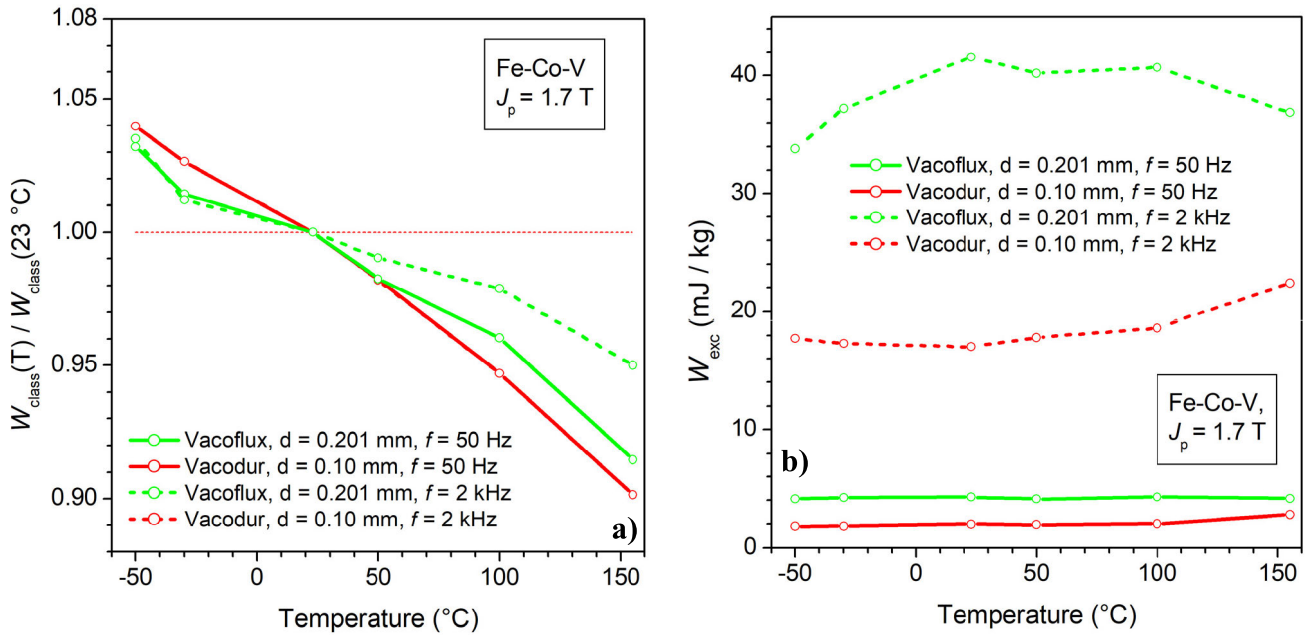
FIGURE 12. a) Classical loss W_{class}(f) , normalized to the value at T = 23 °C, calculated at 50 Hz and 2 kHz as a function of temperature in the Vacoflux and Vacodur sheets. Peak polarization value J_p = 1.7 T. b) Correspondingly obtained excess loss W_{exc}(f) . The skin effect plays a role in the loss decomposition at 2 kHz in the Vacoflux sheets, while weakly affecting the loss in the thinner Vacodur samples.
