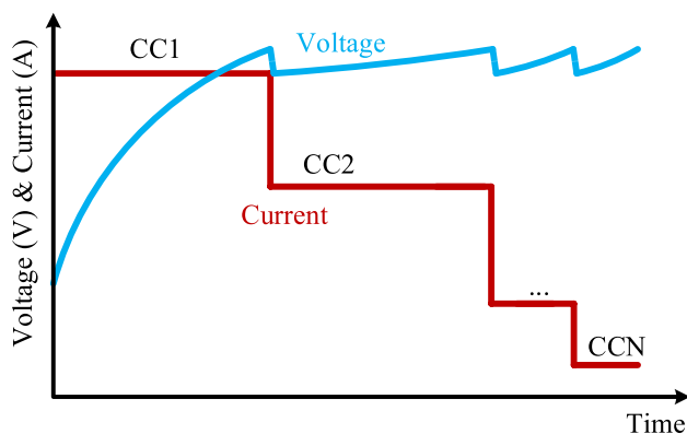
FIGURE 29. MCC charging approach.
