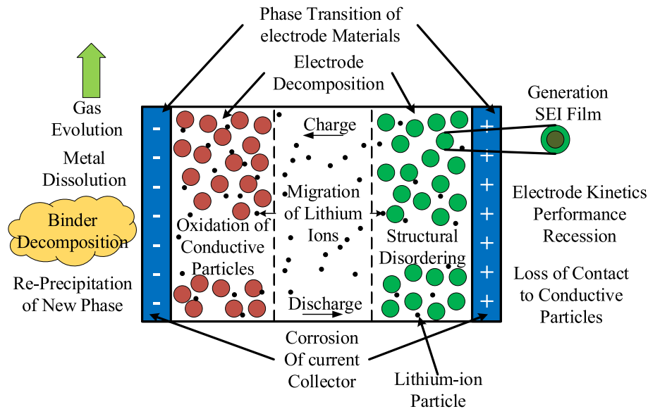
FIGURE 22. Lithium-ion battery aging.
