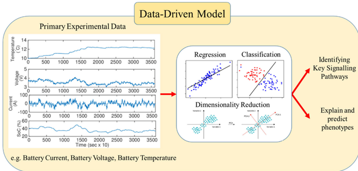
FIGURE 20. Data-driven model [237], [238].
