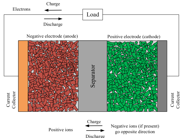
FIGURE 3. Schematic diagram of Li-ion cell.
