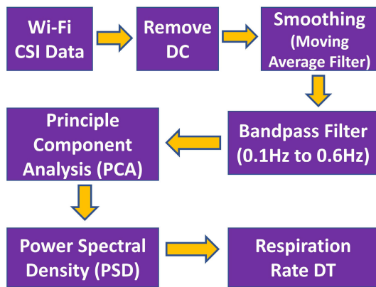
FIGURE 5. Block diagram of pre-processing raw respiration Wi-Fi CSI data.
