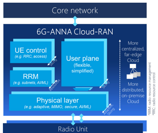
FIGURE 3. 6G-ANNA cloud-RAN components.
