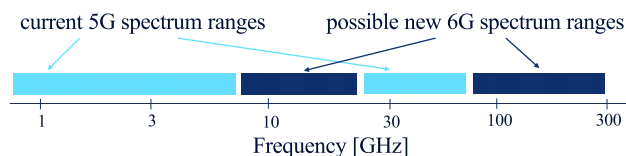
FIGURE 2. Spectrum range for future 6G radio access, illustrating spectrum already available for 5G (cyan) and possible new spectrum for 6G (dark blue).
