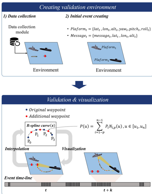
FIGURE 5. Brief description of the scenario for maneuver validation of a submarine.
