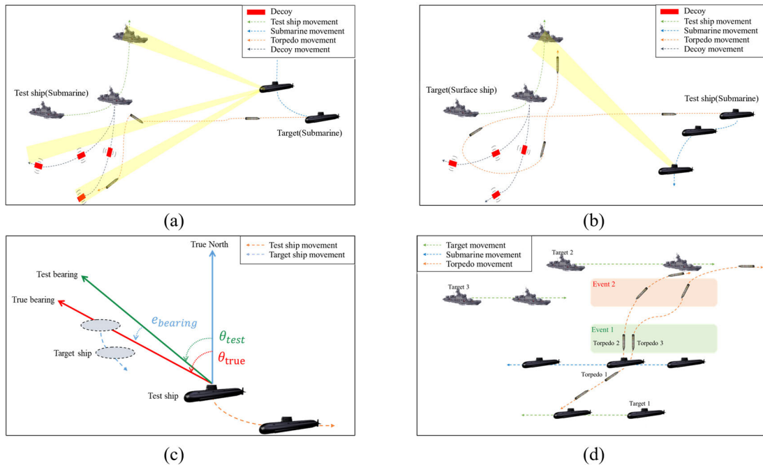
FIGURE 11. Schematics of experimental scenarios. (a) Submarine operation including attack tactics of launching fire-and-forget and wire-guided torpedoes. (b) Surface ship operation including defensive tactics such as launching countermeasures, and evasive maneuvering. (c) Bearing accuracy evaluation. (d) Engagement procedure evaluation using multiple wire-guided torpedoes.
