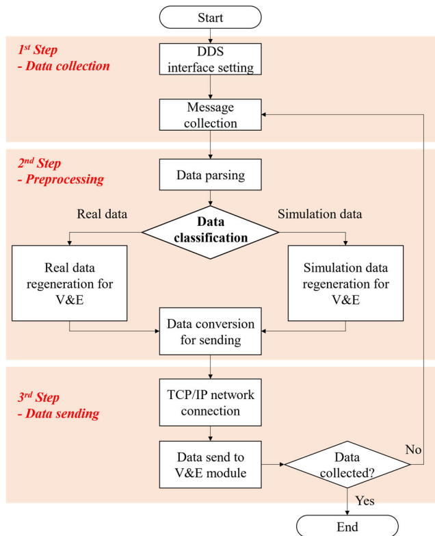
FIGURE 4. Operational flowchart of the data collection module.
