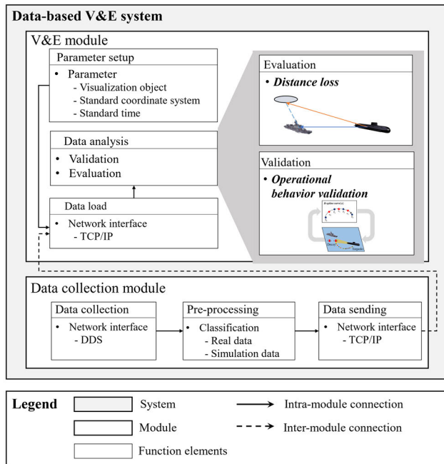
FIGURE 3. Overall DVES configuration.
