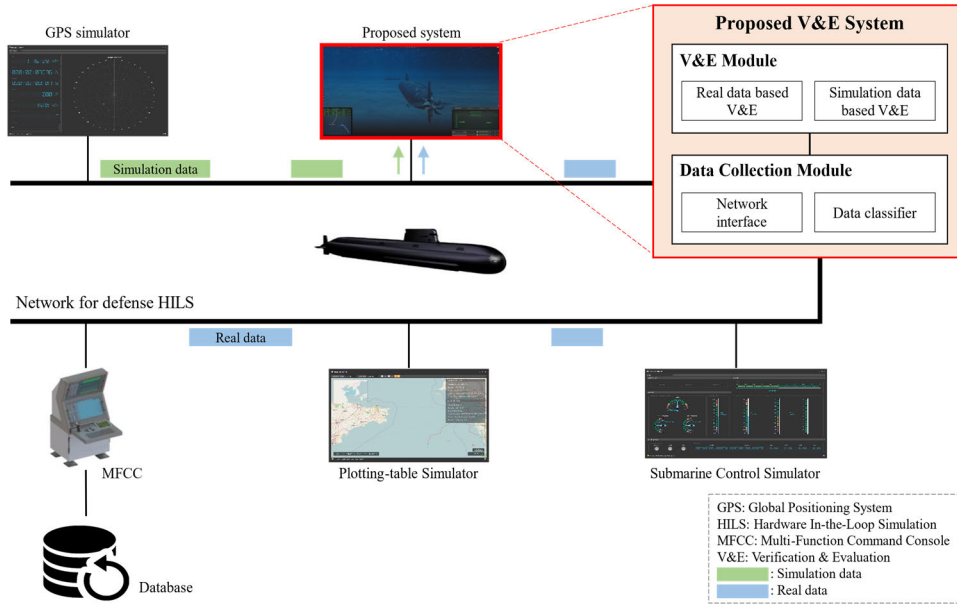
FIGURE 2. Schematic of the proposed DVES for combat system engineering.
