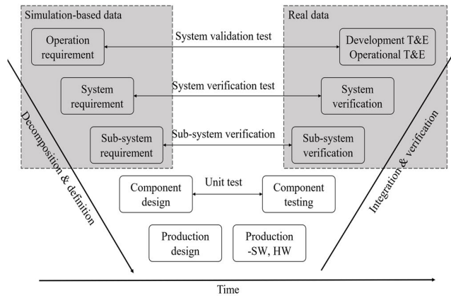
FIGURE 1. V&E application to system engineering.
