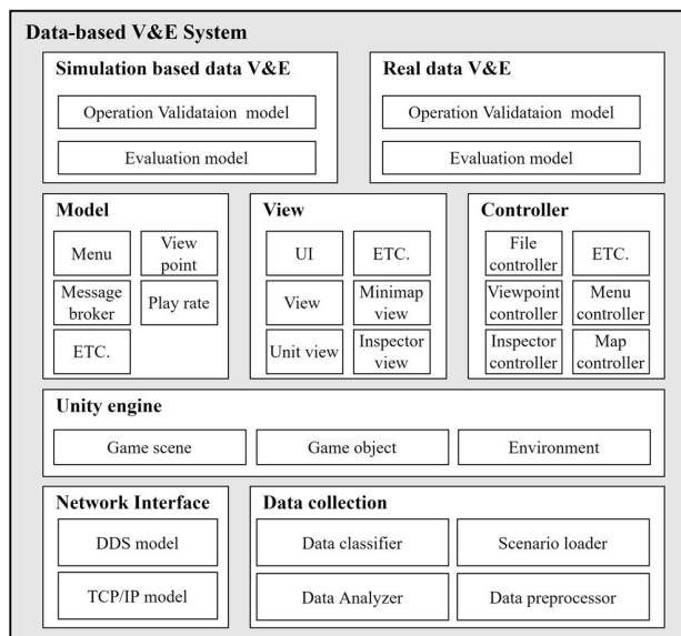
FIGURE 8. Architecture for DVES implementation.
