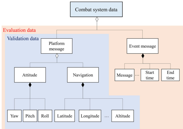
FIGURE 7. Message modeling diagram for combat system engineering.
