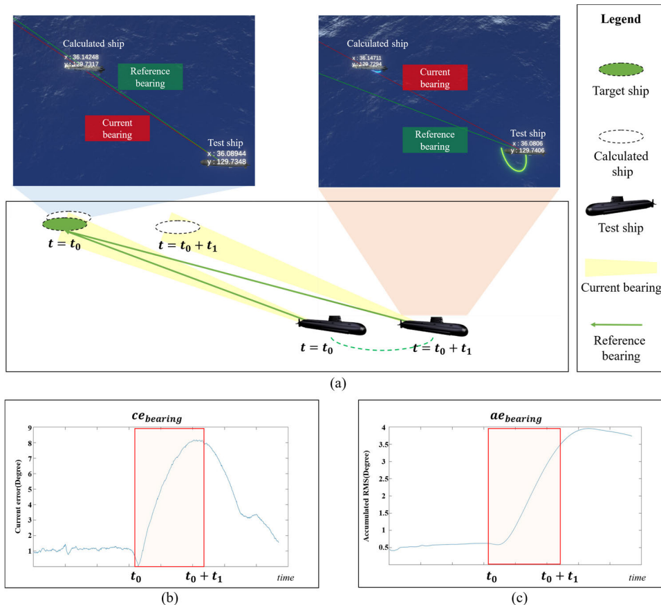
FIGURE 14. DVES screenshots for measuring the bearing accuracy of sensors. (a) Evaluation scenario for radar's accuracy. (b) Measured evaluation loss ( ce_{bearing} ) of radar. (c) Measured total evaluation loss ( ae_{bearing} ) of radar.
