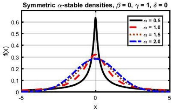
FIGURE 1. Symmetric alpha stable distributions with varying alpha ( \alpha ).
