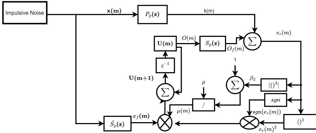
FIGURE 2. Proposed FxRNLMAT algorithm-based ANC system.
