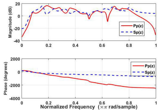
FIGURE 3. Frequency response of primary and secondary acoustic paths.
