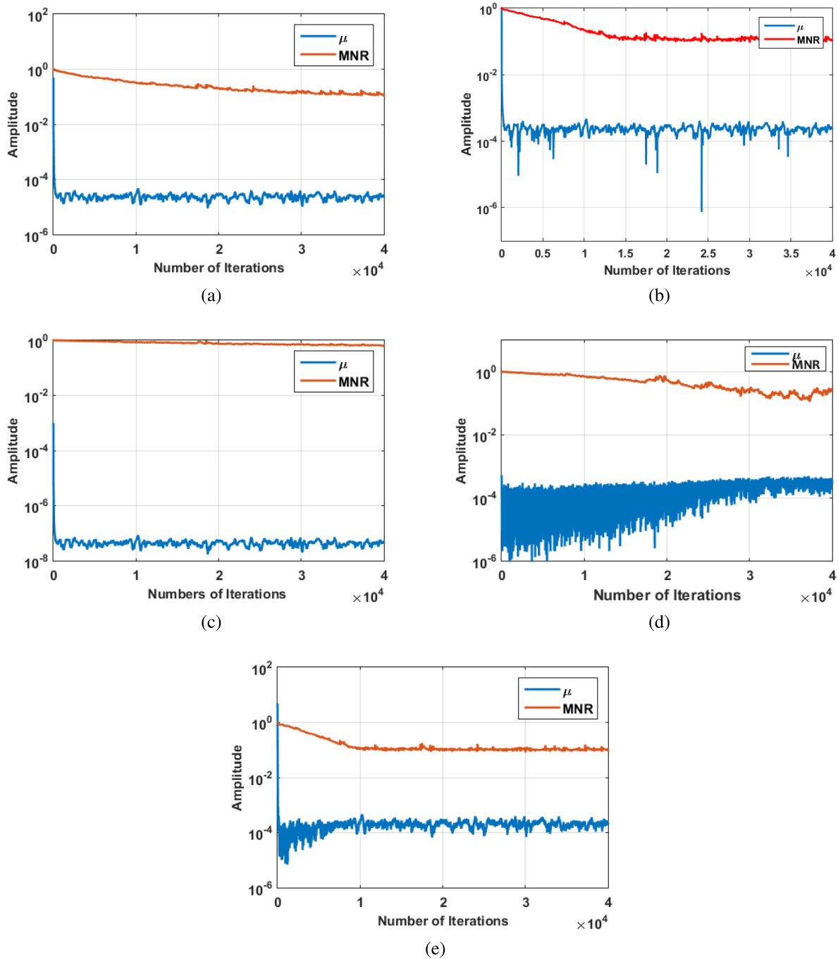
FIGURE 6. Comparison of varying step size and MNR for a) NSSFxLMS (b) MFxLCH (c) Proposed VSSFxLMAT (d) Proposed FxRNLMAT (e) Proposed MFxRNLMAT algorithms.
