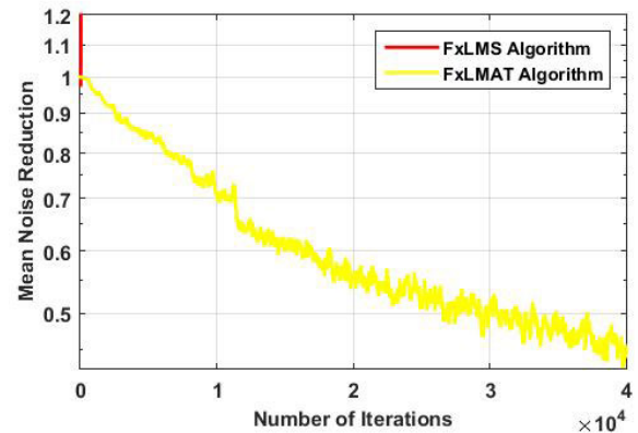
FIGURE 7. MNR curves evaluation for FxLMAT and FxLMS algorithm for case1.
