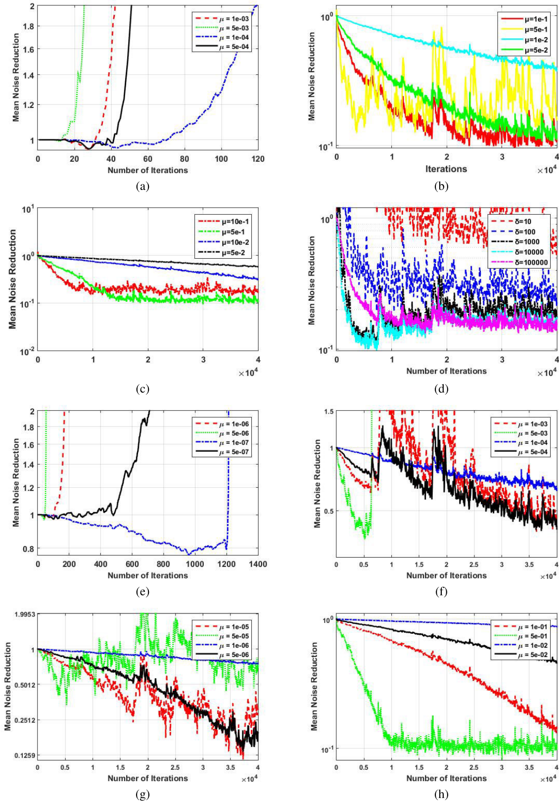
FIGURE 5. MNR curves for case 2 (a) FxLMS algorithm, (b) NSSFxLMS algorithm, (c) MFxLCH algorithm, (d) MGFxRLS algorithm, (e) FxLMAT algorithm, (f) Proposed VSSFxLMAT algorithm, (g) Proposed FxRNLMAT algorithm, (h) Proposed MFxRNLMAT algorithm.
