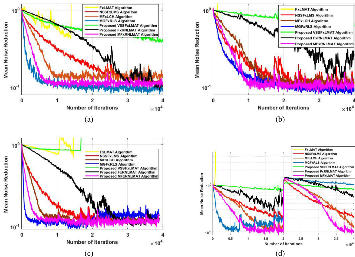
FIGURE 8. MNR curve evaluation of proposed algorithms (a) case-1 (b) case-2, (c) case-3 (d) case-4.
