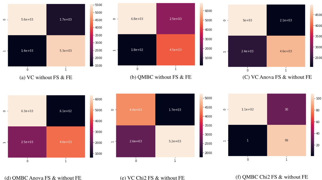
FIGURE 15. The figure presents a grid of subplots illustrating the performance of ensemble models (VC & QMBC) on the CVD Dataset: (a) VC model on the preprocessed (S1) dataset, (b) QMBC model on the preprocessed (S1) dataset, (c) VC model on Anv (S2) dataset without FE, (d) QMBC model on Anv (S2) dataset without FE, (e) VC model on Chi-Square (S3) dataset without FE, (f) QMBC model on Chi-Square (S3) dataset without FE.
