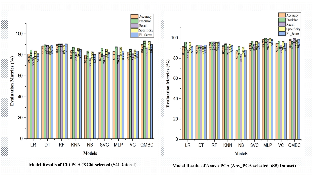
FIGURE 12. Model results of FS & FE technique on HD dataset (Comprehensive.)
