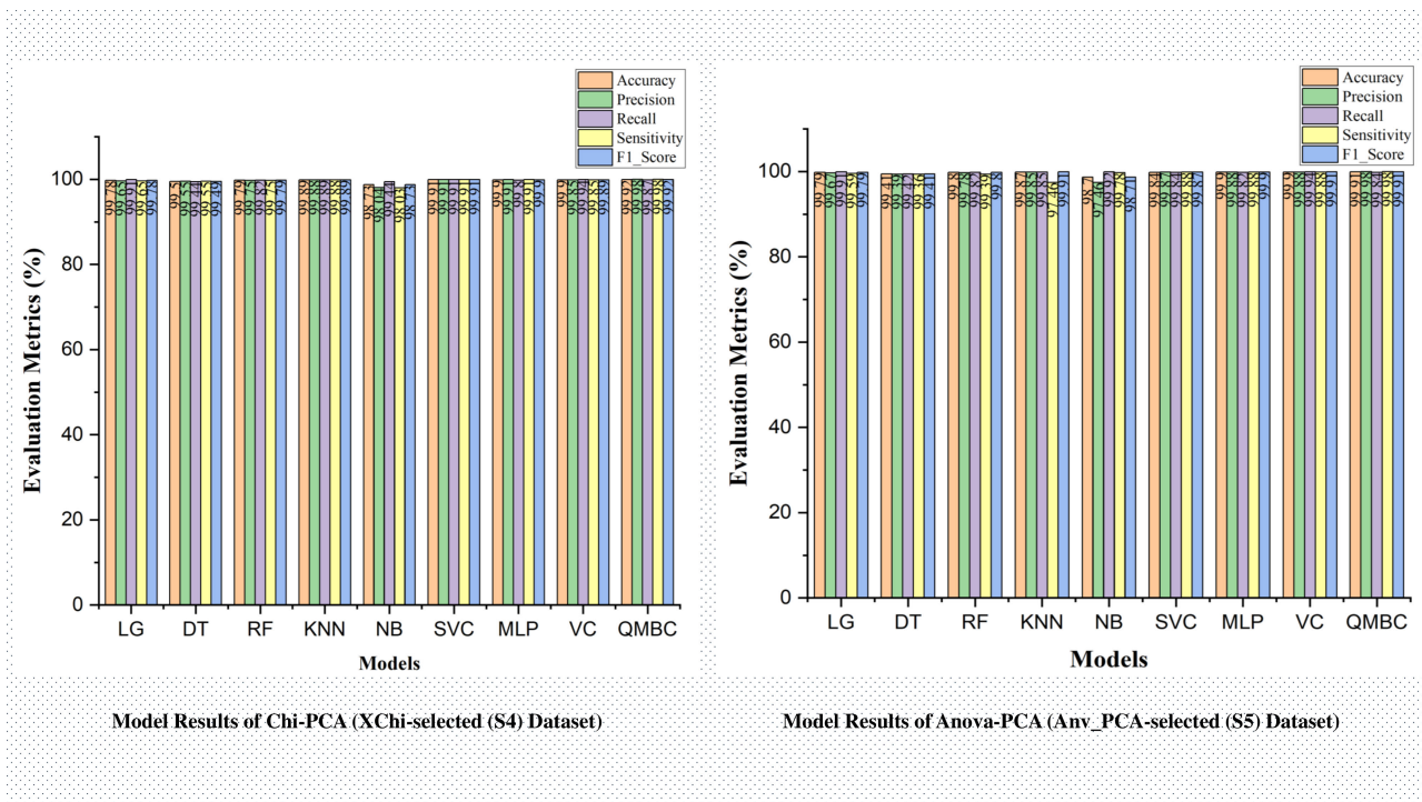
FIGURE 11. Model results of FS & FE technique on CVD dataset.
