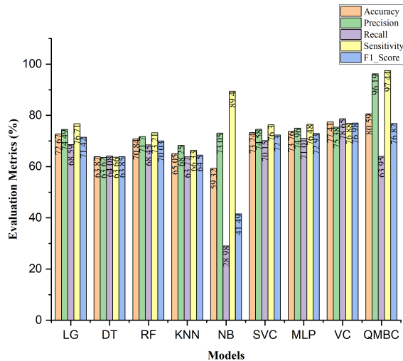
FIGURE 5. Model results of preprocessed (S1) CVD dataset.
