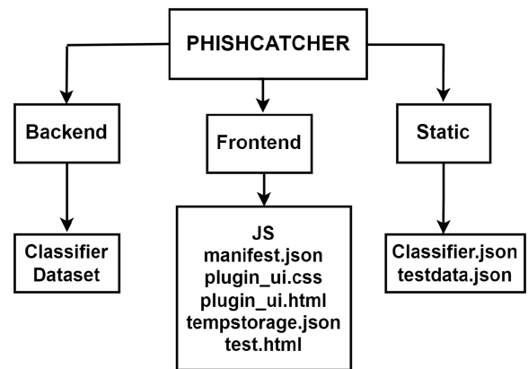
FIGURE 5. PhishCatcher architecture.
