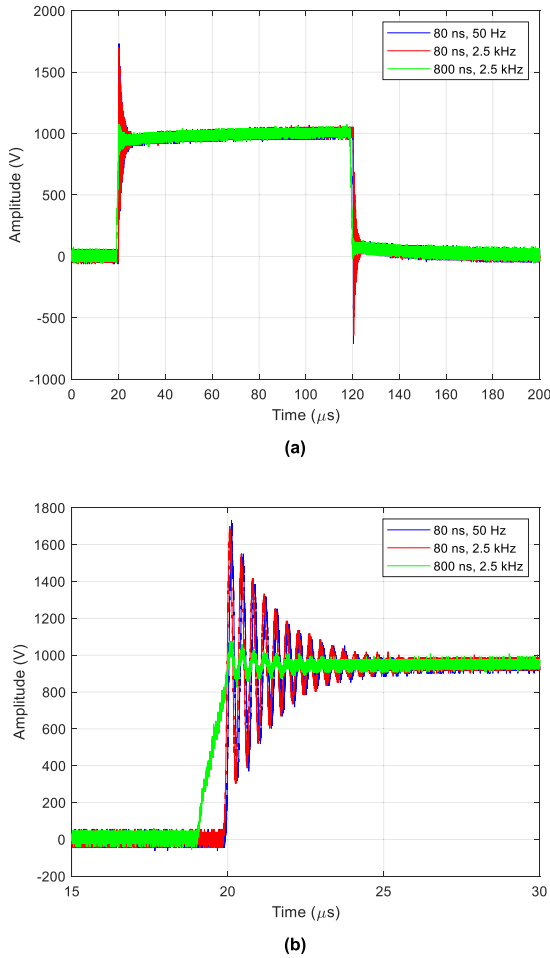
FIGURE 7. (a) The unipolar positive square wave excitations in time domain, and (b) zoom-in waveforms of the rising flanks.
