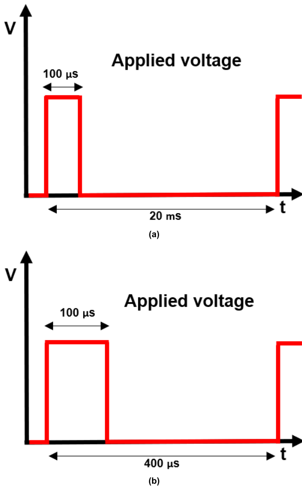
FIGURE 5. Schematic diagrams of applied square waveforms excitations with the constant pulse width of 100 \mu\text{s} corresponding to (a) 50 Hz and (b) 2.5 kHz.
