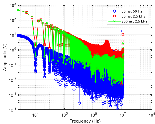
FIGURE 8. FFT of the unipolar square waveforms with two frequencies (50 Hz and 2.5 kHz) and two rise times (80 and 800 ns) at a constant DC voltage equal to 1 kV.
