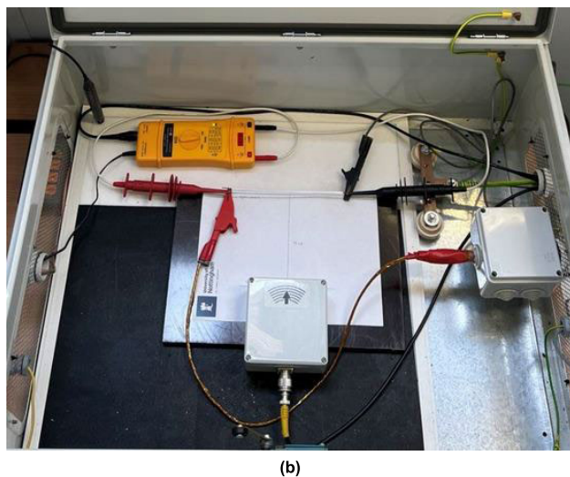
FIGURE 4. (a) PD detection arrangement and (b) Test cell.
