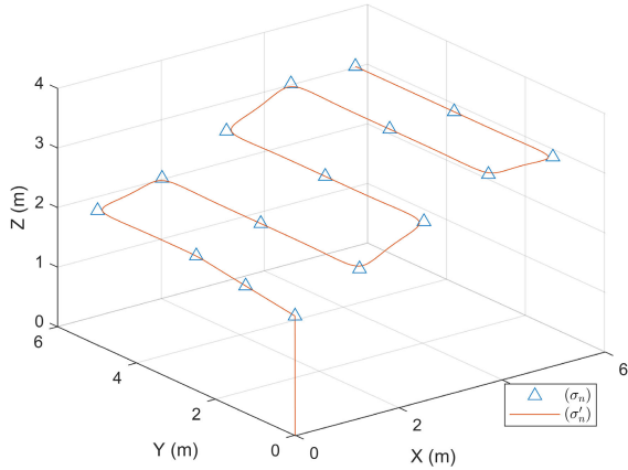
FIGURE 8. The result of local motion planning of flying behavior in (\beta_n), n \in \mathbb{Z} \cap [1, 16] of UAV \alpha_{i,1} performing the search task T_1 .
