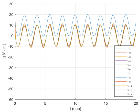
FIGURE 18. The actuator control input u'(t) of the robot \alpha_{1,5} .
