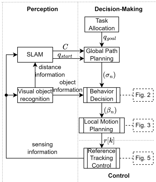
FIGURE 1. The system architecture of S&R tasks in hybrid URTS. In the figure, the three capabilities required for unmanned systems are marked, i.e., perception, decision-making and control. The 2 blocks on left hand side are used to convert the low-level sensor information into high-level information. The Simultaneous Localization And Mapping (SLAM) block converts sensor information and distance information into the current configuration q_{start} of agents and an occupancy map C of URTS. The visual object recognition block provides distance information and object information through the analysis of sensor information. The object information provides agent machine vision that enables it to determine an appropriate behavior (e.g., a robot can see an obstacle and decide to climb through it). The 5 blocks on right hand side are the flowchart of an agent performing a S&R task. From the top to the bottom, it is the decision of the goal configuration q_{goal} of agents, the planning of the path (\sigma_n) of agents, the decision of the behavior (\beta_n) of agents corresponding to the path, the planning of the reference path r[k] of agents corresponding to the behavior, and the low-level reference tracking control of agents. A block with two vertical lines inside in flowchart represents a predefined process which has more detailed subprocesses. Behavior Decision block is described detailly in Fig. 2. Local Motion Planning block to generate the desired reference is described detailly in Fig. 3. Reference Tracking Control block is described detailly in Fig. 5.
