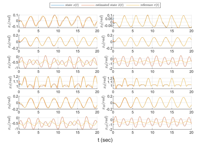
FIGURE 20. The trajectories of reference r(t) , state x(t) and estimated state \hat{x}(t) of the robot \alpha_{1,5} by the traditional PID computed torque controller without FTC [33].
