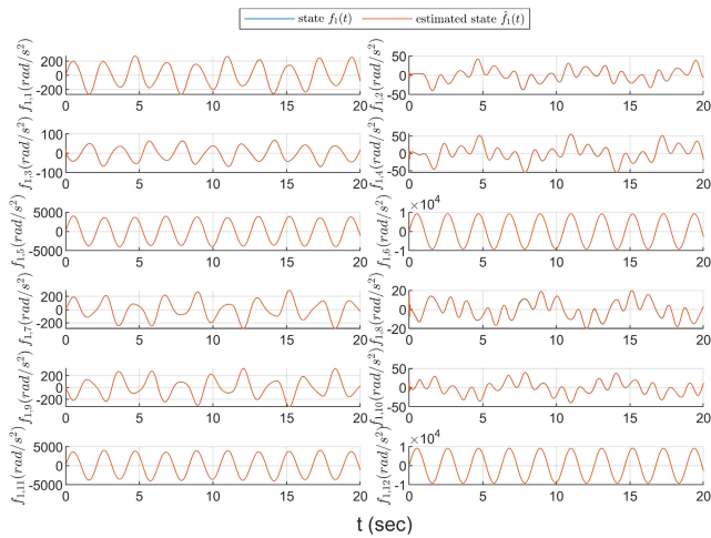
FIGURE 16. The estimation of components of actuator fault f_1(t) of the robot \alpha_{1,5} .
