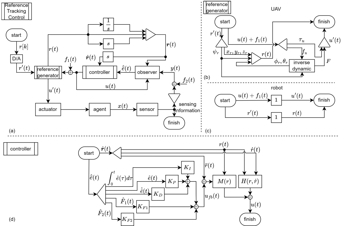
FIGURE 5. (a) The flowchart of Reference Tracking Control block in Fig. 1 of each agent in hybrid URTS. The controller block is described in (d). The controller block (the proposed general H_\infty decentralized observer-based feedforward reference tracking FTC scheme) is designed for a fully actuated agent dynamic model in (8) while the UAV is an underactuated system. It makes the designed feedforward linearization control law u(t) \in \mathbb{R}^6 and the actuator control input u'(t) \in \mathbb{R}^4 different for UAV. The reference generator block is introduced to deal with this problem. For UAVs, the reference generator block is described in (b). For robots, the reference generator block is described in (c). (b) The reference generator block for each UAV. u'(t) and r(t) can be calculated from u(t) and r'(t) by inverse dynamic through the UAV dynamic model in (3). (c) The reference generator block for each robot. u'(t) = u(t) and r(t) = r'(t) since the robot dynamic model in (4) is fully actuated. (d) The proposed general H_\infty decentralized observer-based feedforward reference tracking FTC scheme for each agent in hybrid URTS.
