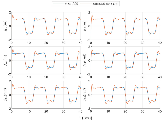
FIGURE 13. The estimation of components of sensor fault f_2(t) of the UAV \alpha_{1,1} .
