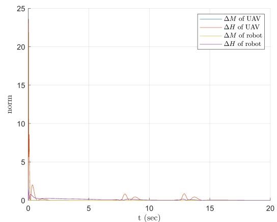
FIGURE 21. The norm of nonlinear terms \Delta M and \Delta H of UAV \alpha_{1,1} and robot \alpha_{1,5} in the first 20 seconds.
