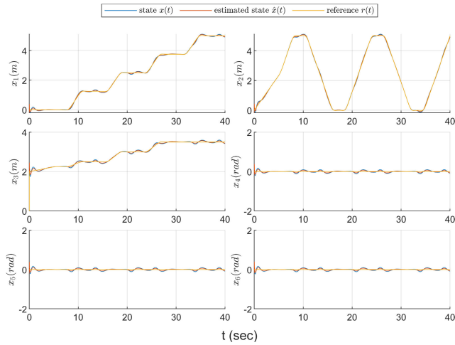
FIGURE 11. The trajectories of components of reference r(t) , state x(t) and estimated state \hat{x}(t) of the UAV \alpha_{1,1} .
