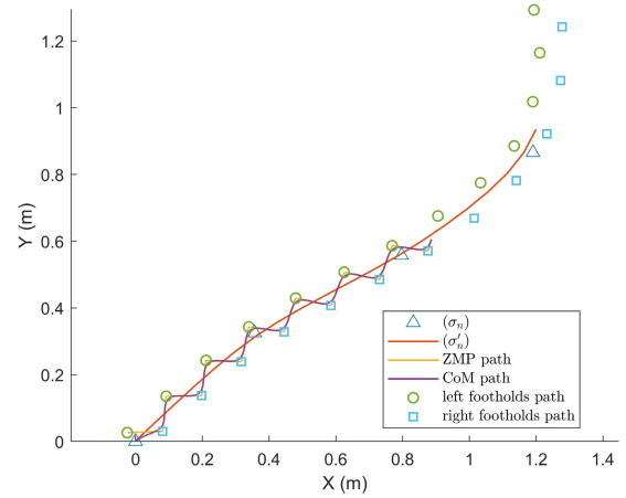
FIGURE 10. The top view of result of local motion planning of walking behavior in (\beta_n), n \in \mathbb{Z} \cap [1, 3] of robot \alpha_{i,5} performing the rescue task T_7 . The joint path, i.e., reference path r[k] will be obtained by solving IK with CoM, left foothold and right foothold path.
