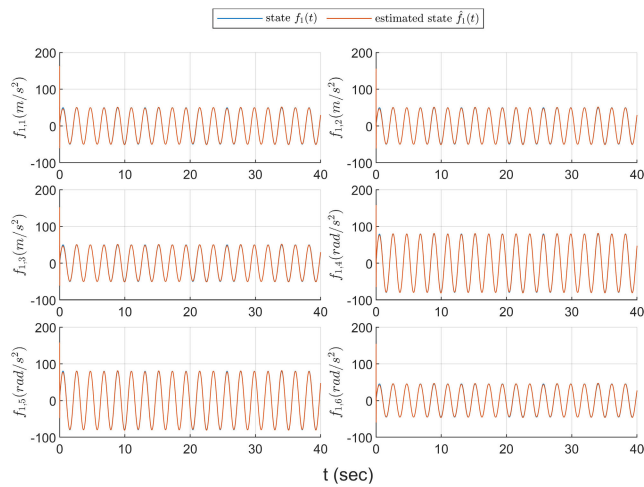
FIGURE 12. The estimation of components of actuator fault f_1(t) of the UAV \alpha_{1,1} .
