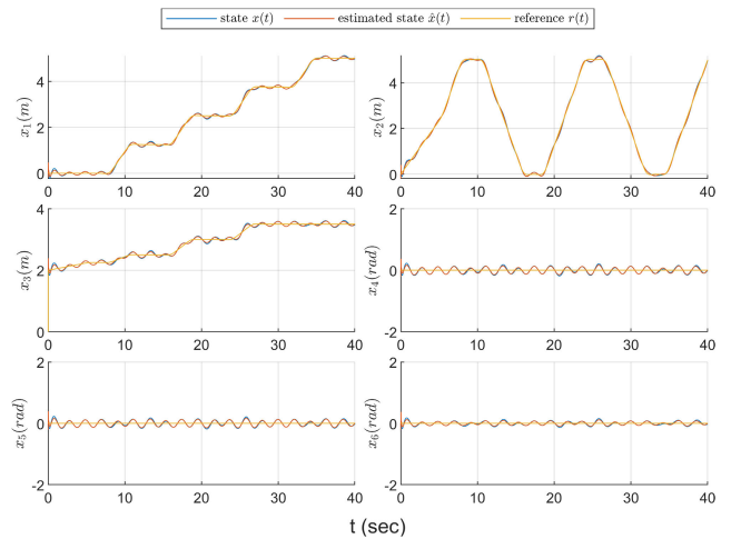
FIGURE 19. The trajectories of reference r(t) , state x(t) and estimated state \hat{x}(t) of the UAV \alpha_{1,1} by the traditional PID computed torque controller without FTC [33].
