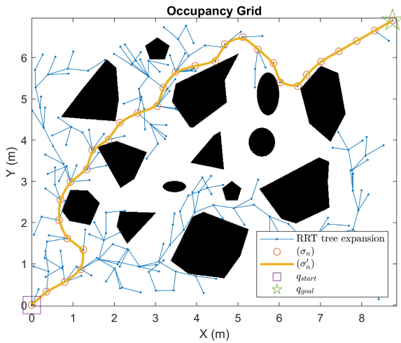
FIGURE 9. The global path planning result of the robot \alpha_{i,5} performing the rescue task T_7 using RRT algorithm. The block polygons represent the safety obstacle space C'_{obs} which takes into account the geometric size of agent's mechanical body.
