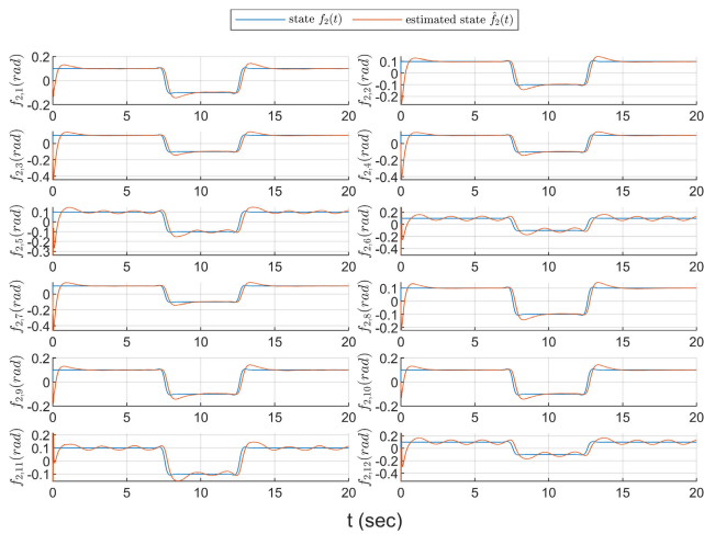
FIGURE 17. The estimation of components of sensor fault f_2(t) of the robot \alpha_{1,5} .
