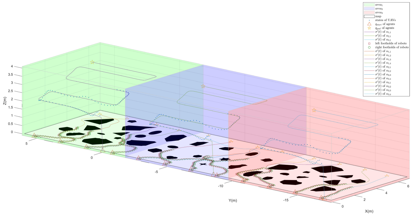
FIGURE 22. The simulation of team tracking of URTS for team_i, i = 1, 2, 3 when they perform search tasks.
