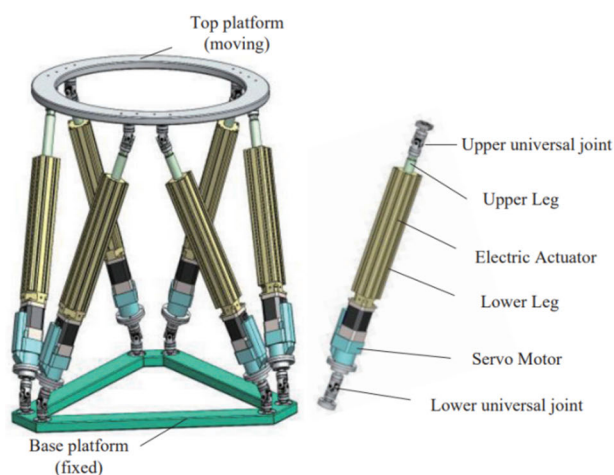
FIGURE 1. Stewart platform [3].
