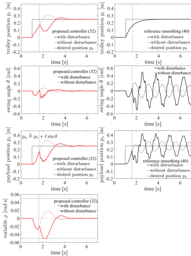
FIGURE 6. Experiment III: PTP control under disturbance. The payload was hit by an external object at the time indicated by the gray vertical lines.
