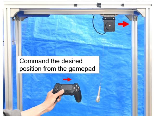
FIGURE 13. Experimental setup of the human operation of the crane.
