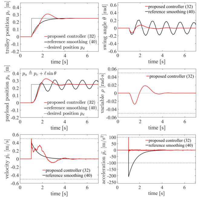
FIGURE 4. Experiment I: point-to-point (PTP) control. The horizontal dotted lines indicate upper bounds of each variable.
