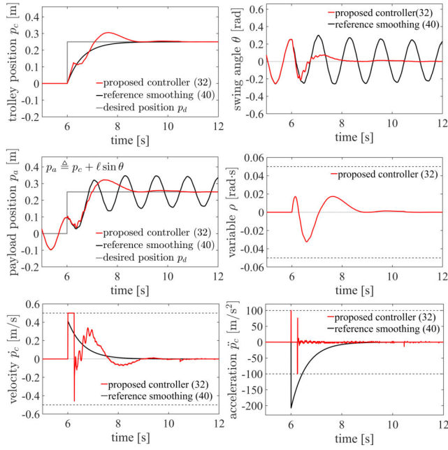
FIGURE 5. Experiment II: PTP control with initial sway. The horizontal dotted lines indicate upper bounds for each variable.
