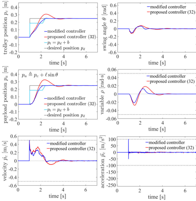
FIGURE 10. PTP Control with the modified controller.
