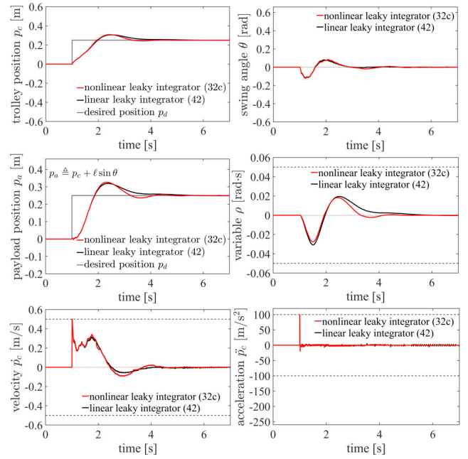
FIGURE 7. Experiment IV: effects of the nonlinear leaky integral controller.
