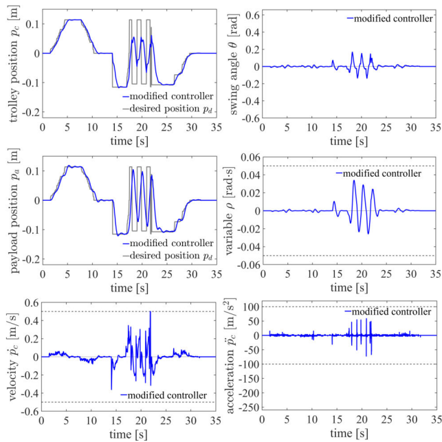
FIGURE 14. Human operation of the crane with the modified controller. Note that the scale of the vertical axis of the trolley position p_c and payload position are not the same as those in other experiments.
