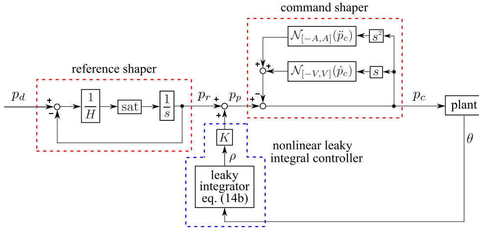
FIGURE 2. Block diagram of the proposed controller.
