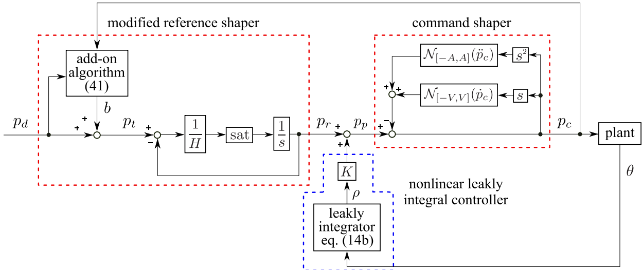
FIGURE 8. Block diagram of the modified controller with the add-on algorithm (41).
