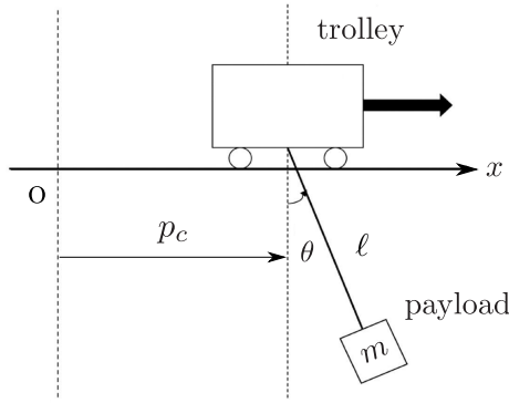
FIGURE 1. Dynamics model of a 2-D overhead crane.
