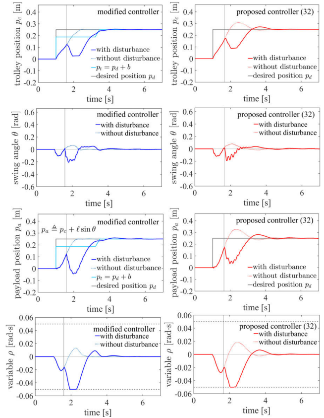
FIGURE 12. PTP Control under disturbance with the modified controller. The payload was hit by an external object at the time indicated by the gray vertical lines.
