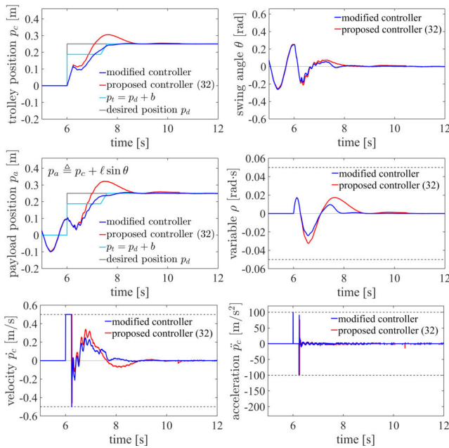
FIGURE 11. PTP Control with initial sway with the modified controller.
