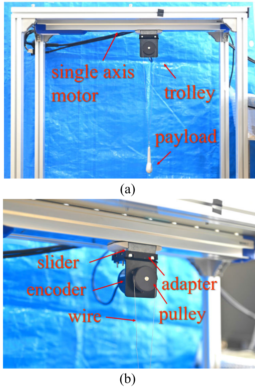
FIGURE 3. Laboratory setup: (a) 2-D overhead crane, (b) configuration of the trolley.
