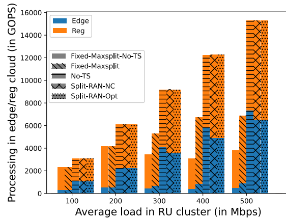
(b) Processing in edge and regional cloud
