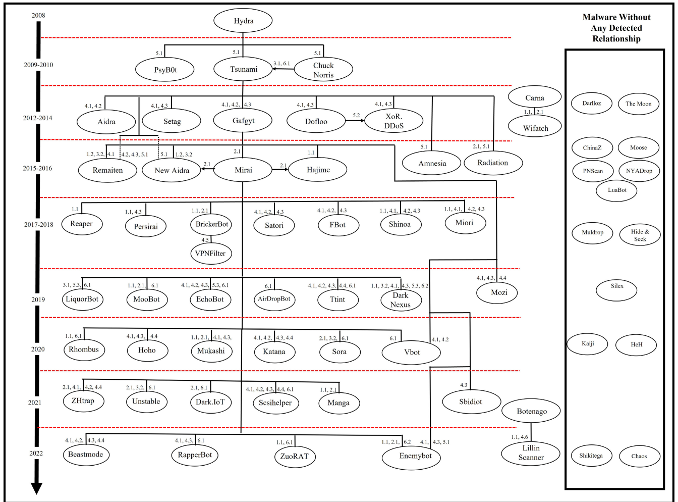
FIGURE 5. Phylogenetic tree of IoT malware families.
