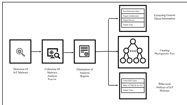
FIGURE 1. General overview of methodology.
