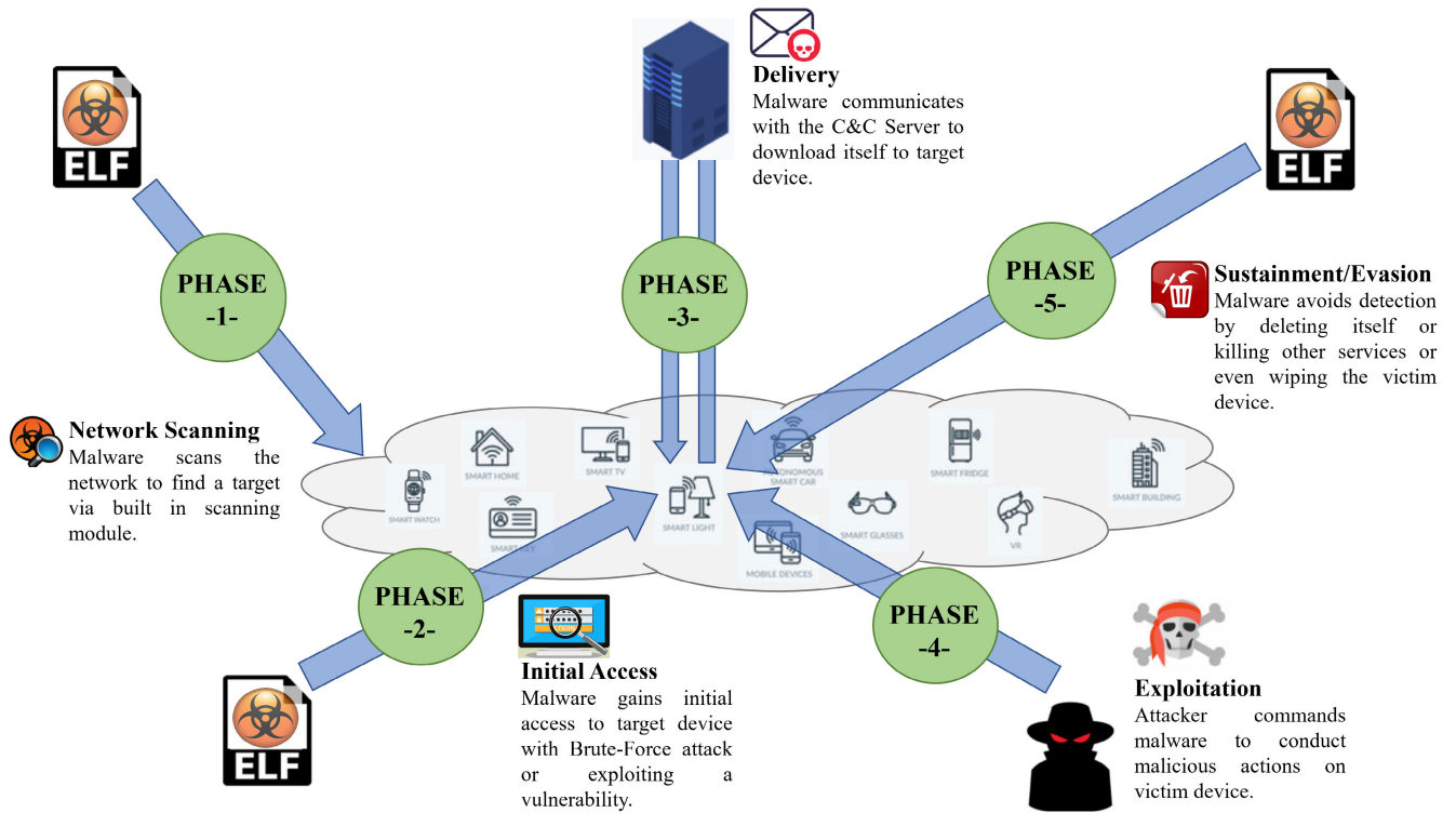
FIGURE 6. Common threat pattern of IoT malware families.
