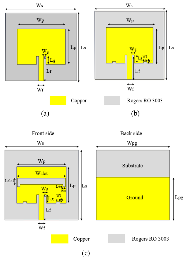
FIGURE 1. The proposed design's evolution (a) CPA (b) CPA with slots (c) proposed antenna.
