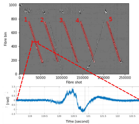
FIGURE 2. Section of DAS collected data (top) for the 50 km/h experiment showing the five target vehicles in addition to two unwanted ones. In addition, a sample DAS signal is taken at bin 450 for Car 1 as shown in the bottom, where 1000.04 fibre shots are presented as one second and the y-axis shows the disturbance level in radians.
