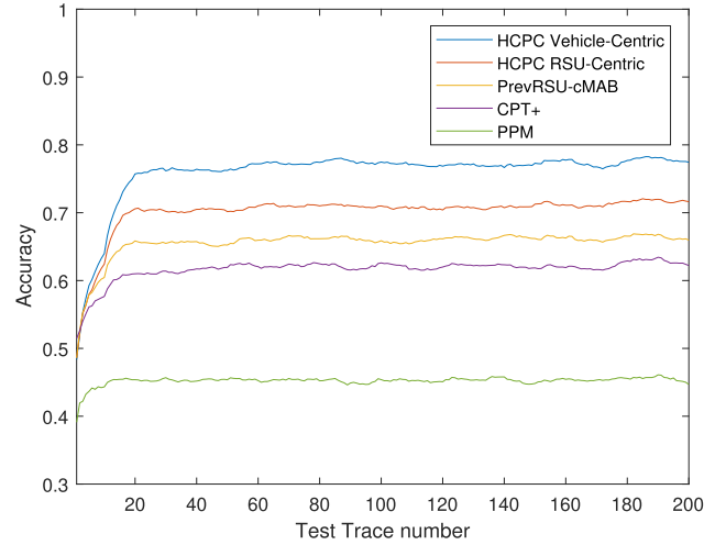
FIGURE 7. Cumulative prediction accuracy of the five proactive caching systems in Manchester - Mixed Traffic Scenario.
