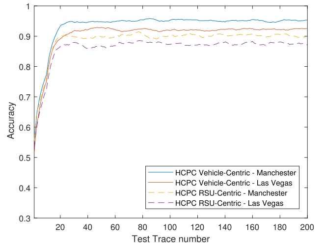
FIGURE 8. Prediction accuracy of the Vehicle-Centric and RSU-Centric hybrid systems showing only commuting vehicles in two cities - Mixed Traffic Scenario.
