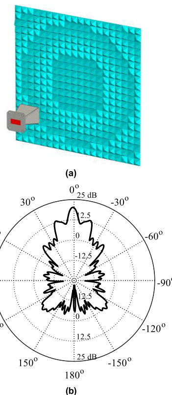
FIGURE 4. 20 \times 20 RA designed using the inverse surrogate model developed for the unit cell of Fig. 2: (a) 3D view of the RA, (b) EM-simulated realized gain at f_0 = 10 GHz.
