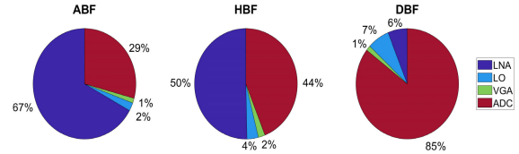
FIGURE 20. ADC power consumption.
