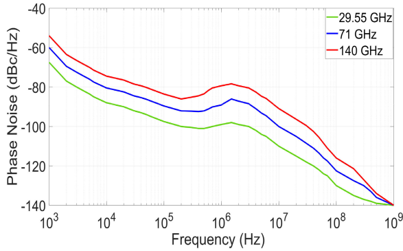
FIGURE 8. Phase noise estimation for PLLs at 71 GHz and 140 GHz.
