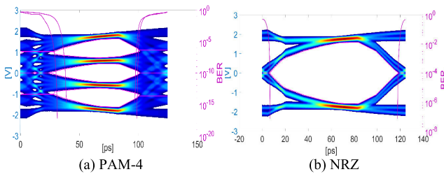
FIGURE 17. DFE Eye diagrams with BER.
