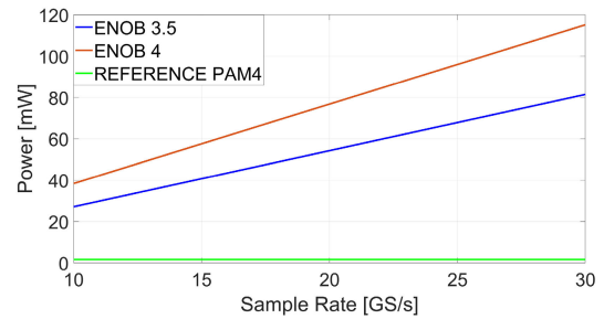
FIGURE 21. Low resolution ADC power consumption.
