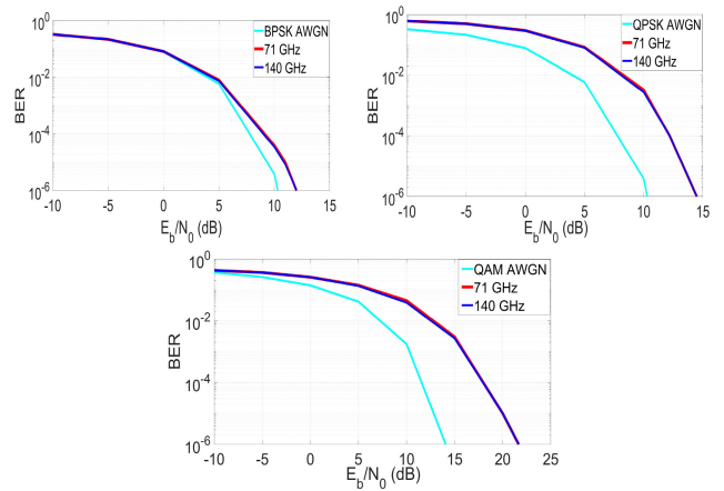
FIGURE 13. LPAP Rx BER curves.
