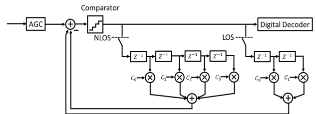
FIGURE 14. DFE for LPAP Rx.
