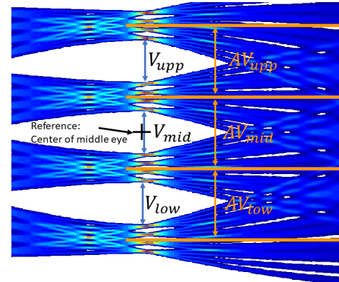
FIGURE 18. Eye measurements.
