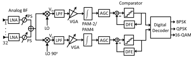
FIGURE 2. LPAP Rx architecture.
