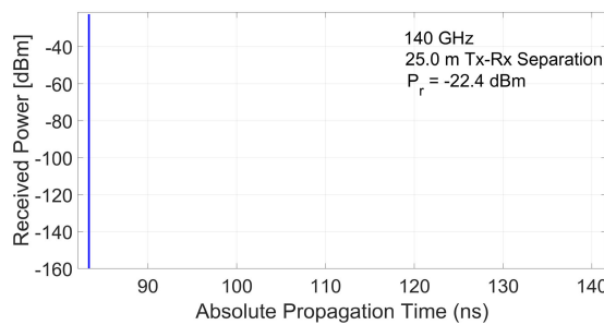
FIGURE 5. PDP 140 GHz channel.
