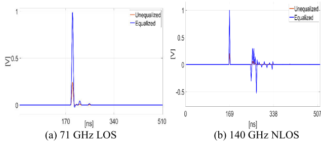
FIGURE 15. DFE Impulse response.
