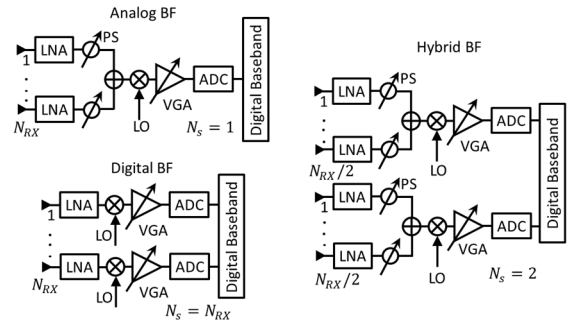
FIGURE 1. Analog, hybrid and digital beamforming.
