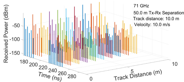
FIGURE 3. PDP 71 GHz channel.
