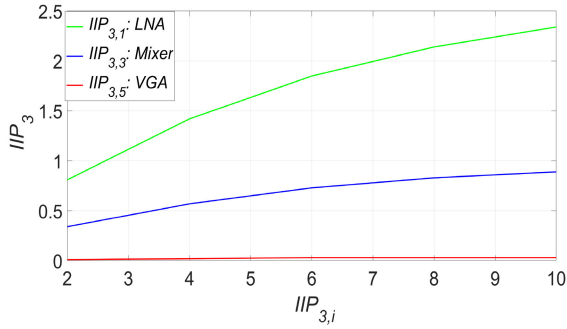
FIGURE 19. SFDR improvement.
