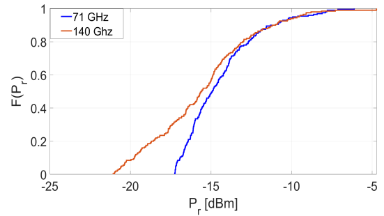
FIGURE 6. Cumulative density function of power received.
