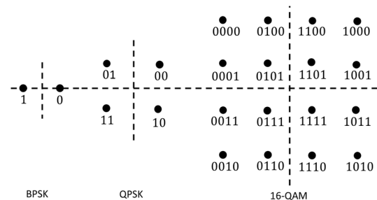
FIGURE 11. Gray mapping and symbols.
