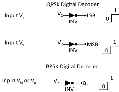
FIGURE 12. Digital decoder for QPSK, BPSK.
