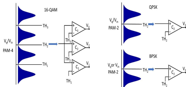
FIGURE 9. Comparator with signal inputs.
