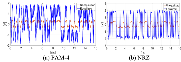
FIGURE 16. PRBS waveform.
