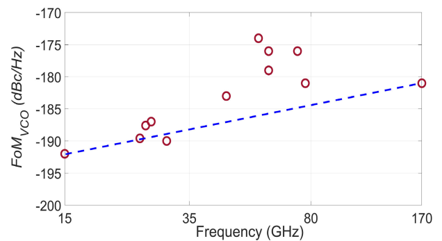
FIGURE 7. FOM_{VCO} for state-of-the art VCOs implemented in CMOS.
