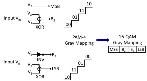
FIGURE 10. Digital decoder for 16-QAM.
