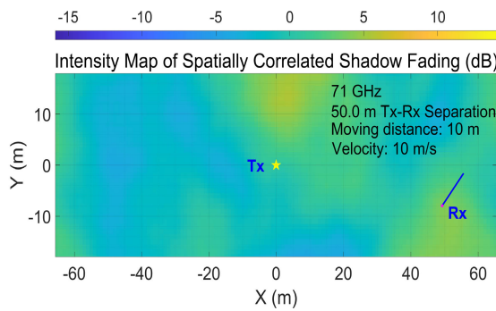
FIGURE 4. 71 GHz channel variation in PDP due to Rx mobility.
