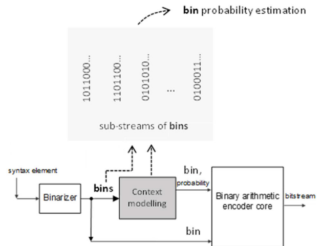
FIGURE 1. Main functional blocks in the CABAC technique.
