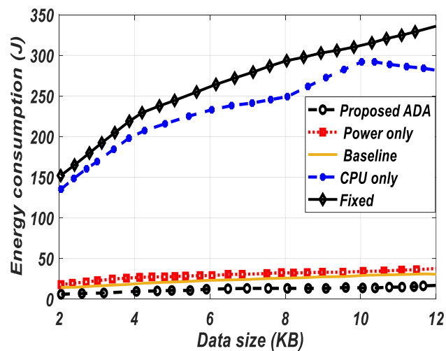
FIGURE 4. Energy consumption related to data size.
