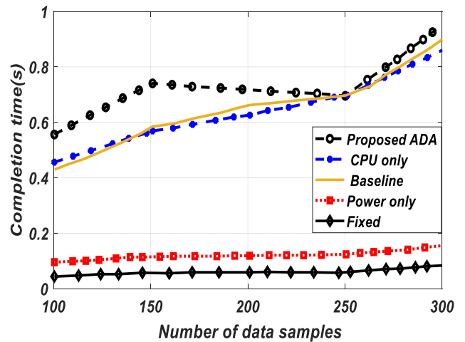
FIGURE 7. Completion time related to number of data samples.
