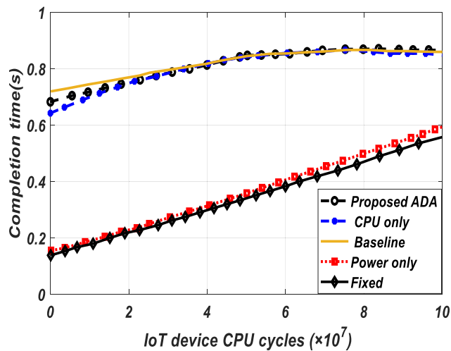
FIGURE 9. Completion time vs CPU cycles.
