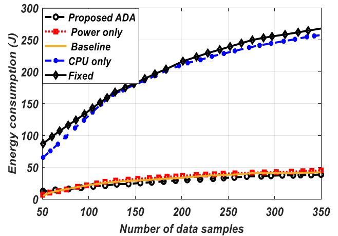
FIGURE 5. Energy consumption vs a number of data samples.
