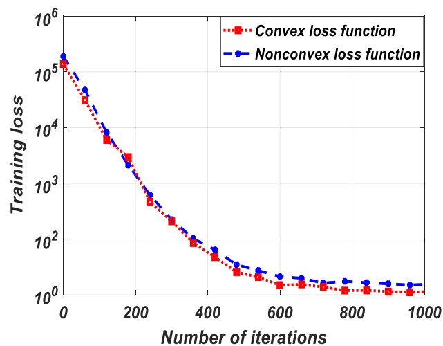
FIGURE 10. Training loss vs number of iterations.
