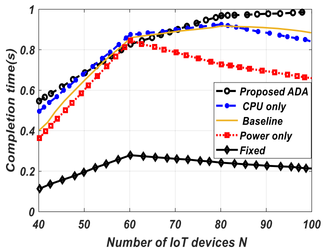
FIGURE 8. Completion time related to number of IoT devices.
