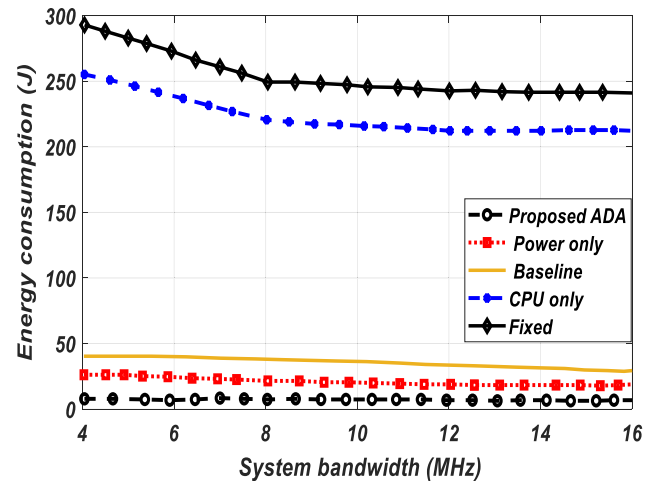
FIGURE 6. Energy consumption related to system bandwidth.
