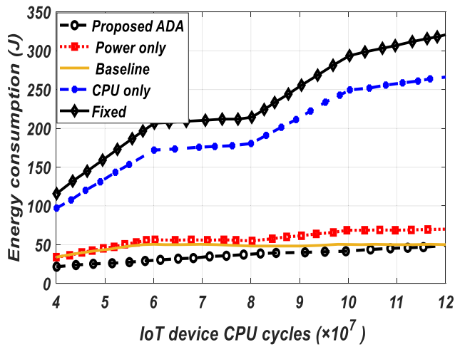
FIGURE 3. Energy consumption related to CPU cycles.
