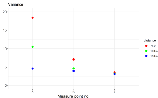
FIGURE 16. Variance of vehicle velocity for distance d equals 75m, 100m, 150m (slippery pavement case). The speed variance at the beginning and middle of the road curve is noticeably higher than for dry pavement (Fig. 6), the speed limits at the preceding points are likely suboptimal.
