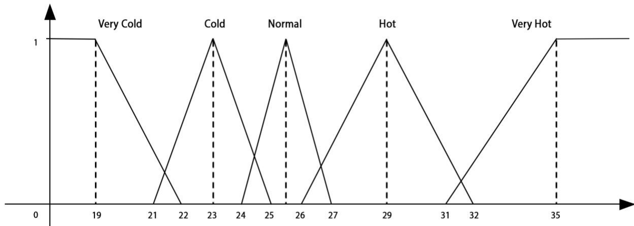
FIGURE 11. Temperature membership function curve.
