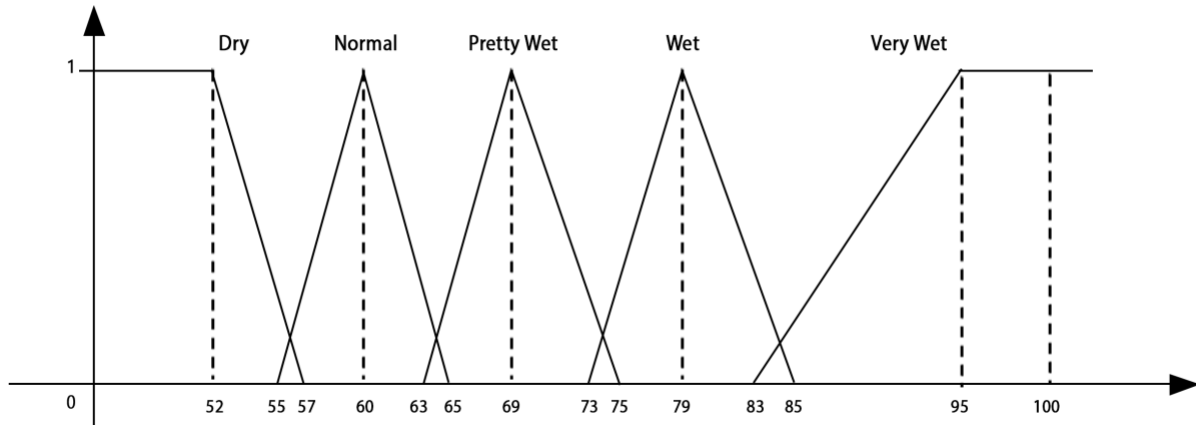
FIGURE 12. Humidity membership function curve.
