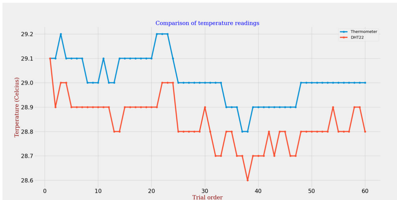
FIGURE 14. Comparison of temperature measurements.
