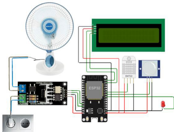
FIGURE 7. Tool design.
