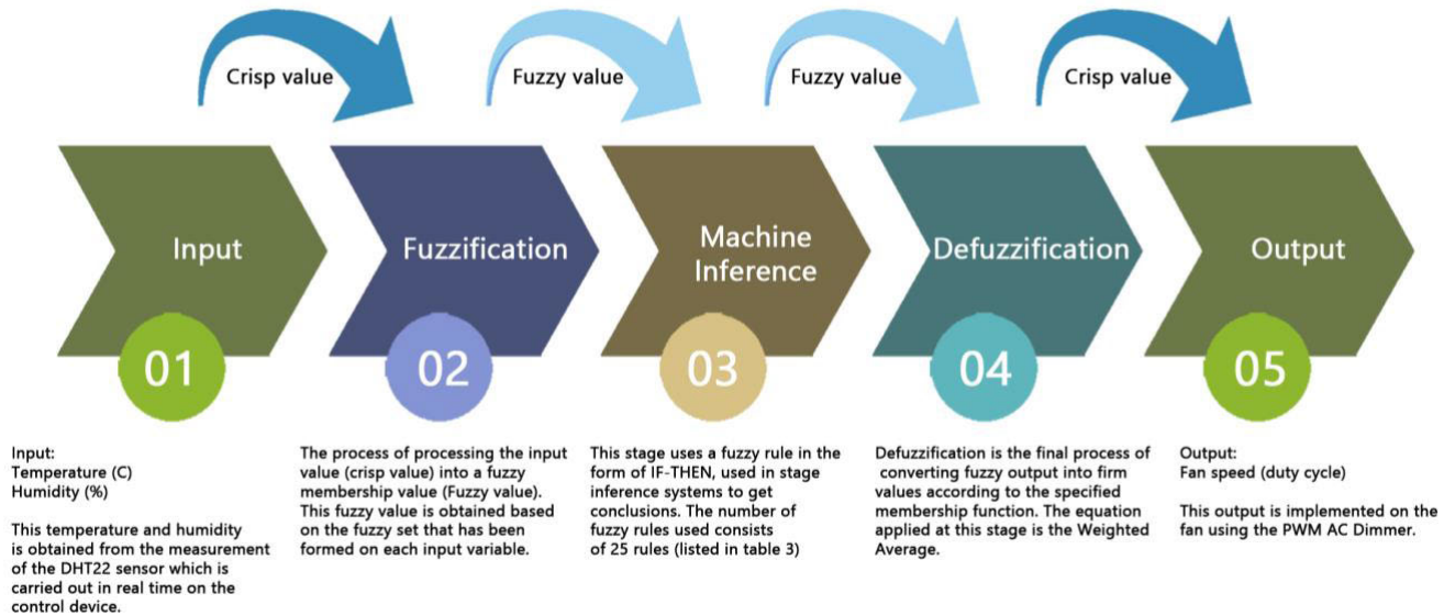
FIGURE 10. Stages of FIS Tsukamoto.
