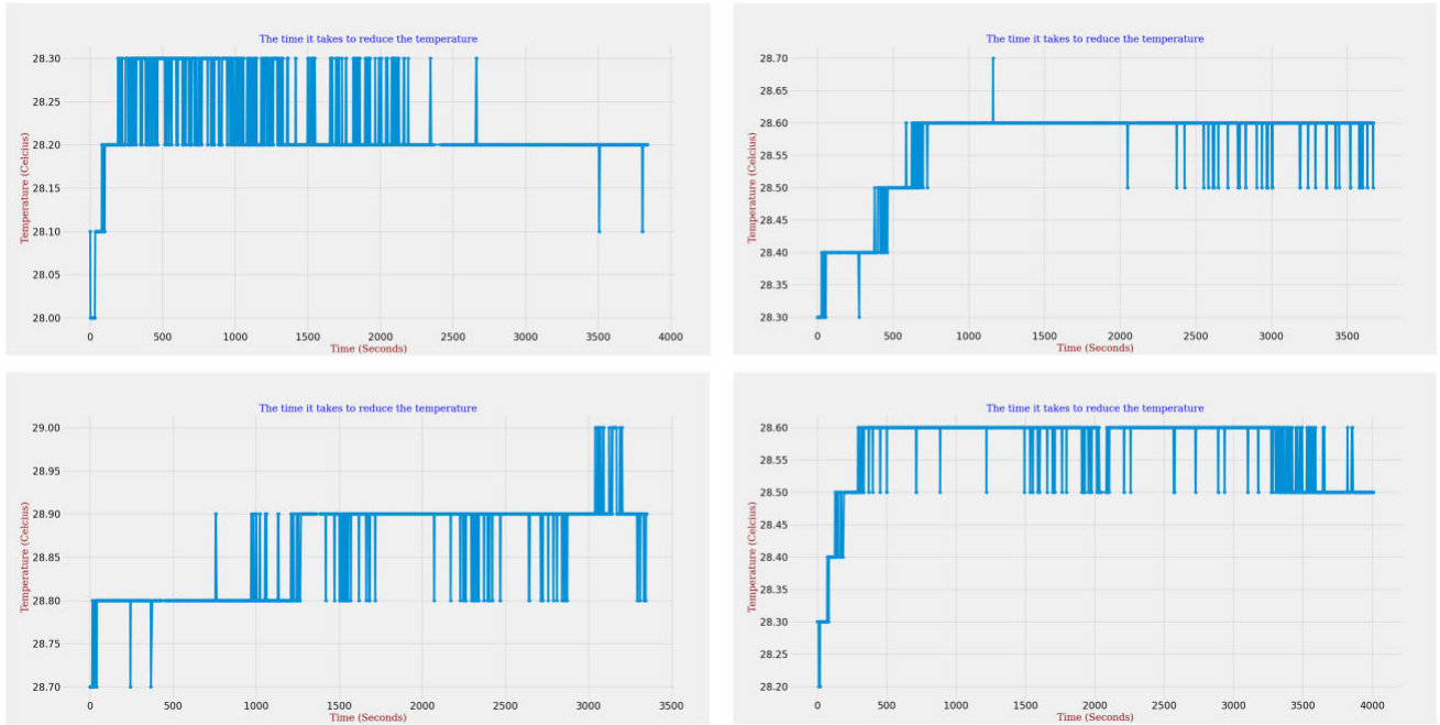
FIGURE 22. Second position test (next to the fan).
