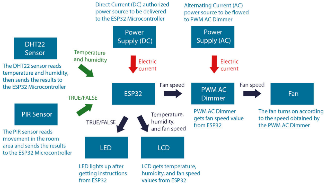
FIGURE 17. Tool working flowchart.
