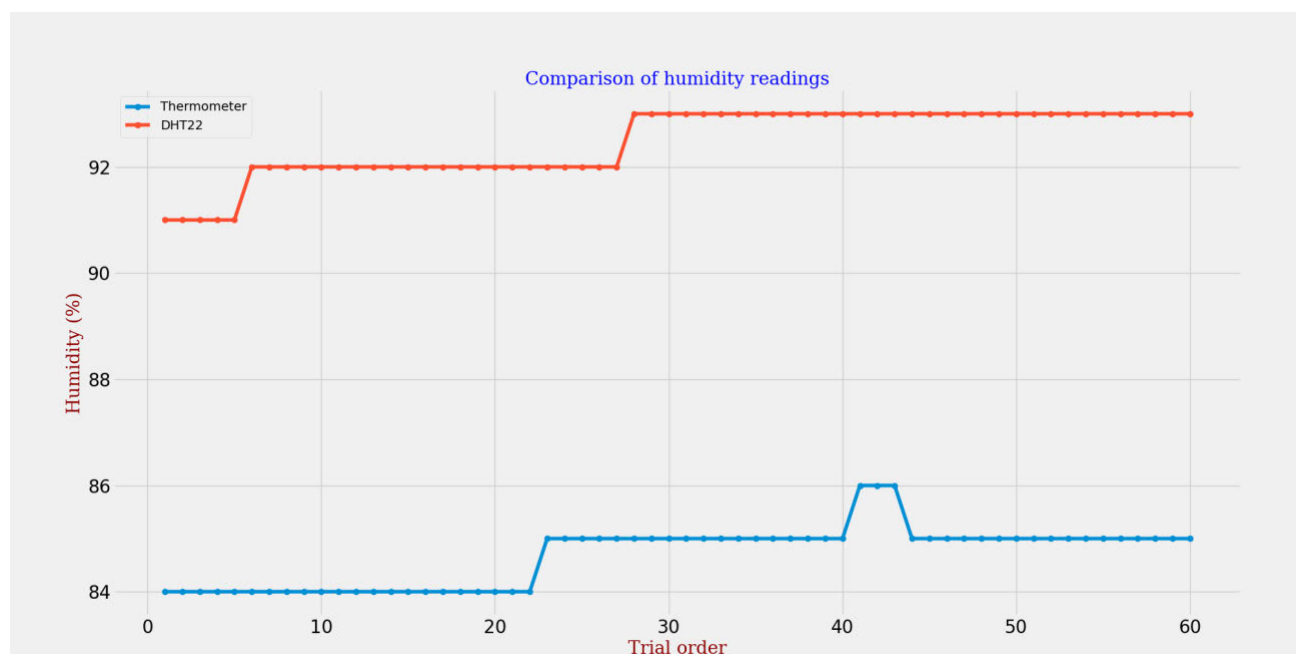
FIGURE 15. Comparison of humidity measurements.
