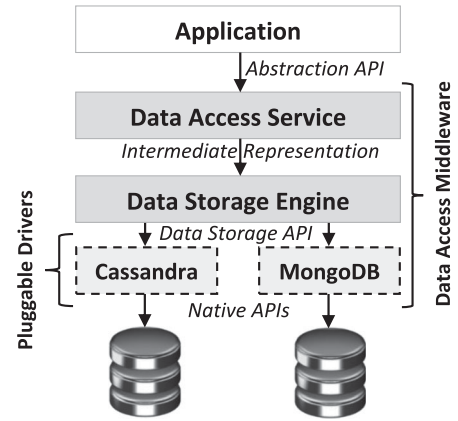
Fig. 1. Typical underlying architecture of data access middleware platforms.
