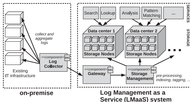
Fig. 2. Logical architecture of the log management as a service (LMaaS) system.
