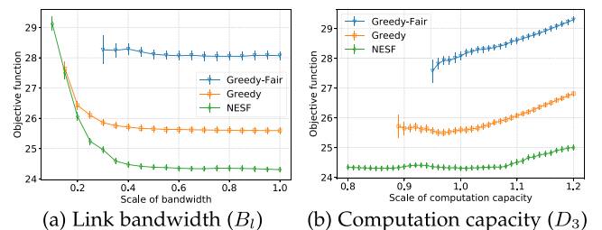
Fig. 7. Selected numerical results for città studi topology.
