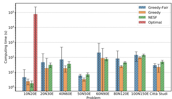
Fig. 13. Computing time.
