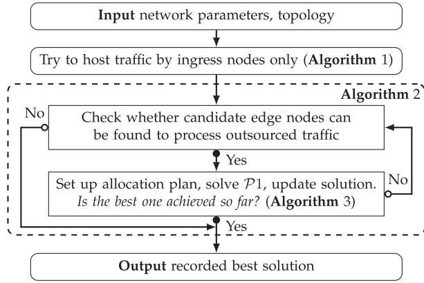
Fig. 4. Flowchart of our NESF heuristic.
