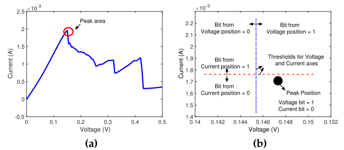
FIGURE 1. (a) I-V characteristic. (b) An example of bit generation process out of an I-V spectrum. Number of bins is selected as 2. Bit numbers of 1 and 0 are generated from voltage and current axes, respectively.
