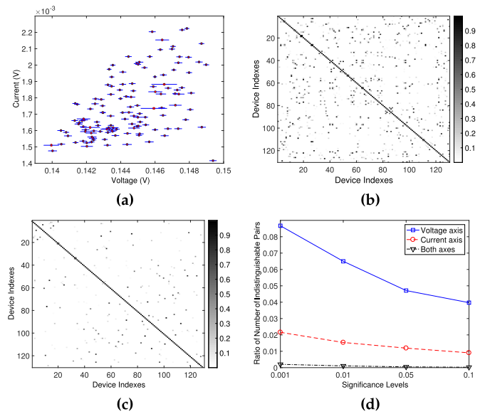
FIGURE 3. (a) Peak locations of the I-V spectrum with error bars on both voltage and current axes, using the mean and 99 percent confidence level of the 50 measurements in high resolution. Individual peaks are clearly discernible. (b), (c) p -values when 130 devices are compared to each other with the peak positions in voltage and current axes, respectively. (d) Ratio of the indistinguishable pairs over the total pairs with varying significance levels on voltage and current axes, and on both axes at the same time.
