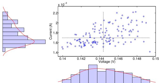
FIGURE 4. Peak positions averaged from 50 measurements in high resolution of 130 devices.
