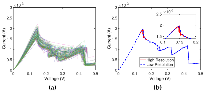
FIGURE 2. I-V spectrum of 130 devices. (a) One measurement for 130 devices in low resolution. (b) 10 and 50 measurements for one device in low and high resolution, respectively.
