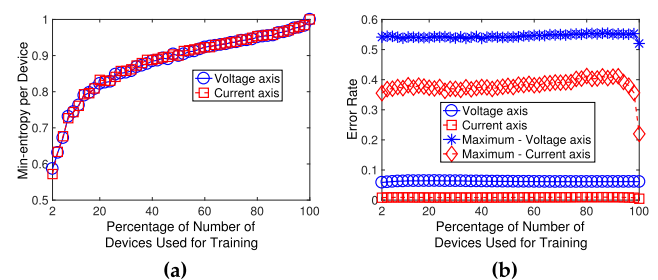
FIGURE 5. (a) Min-entropy amount when using different numbers of devices for training. (b) Error rates when using different numbers of devices for training.
