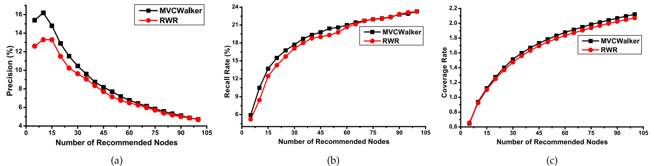
FIGURE 8. Performance of MVCWalker and Basic RWR over Number of Recommended Nodes. (a) Precision. (b) Recall Rate. (c) Coverage Rate.
