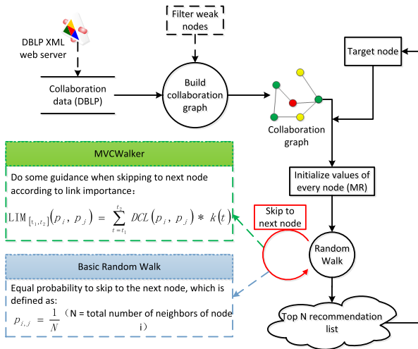
FIGURE 2. Structure of MVCWalker.
