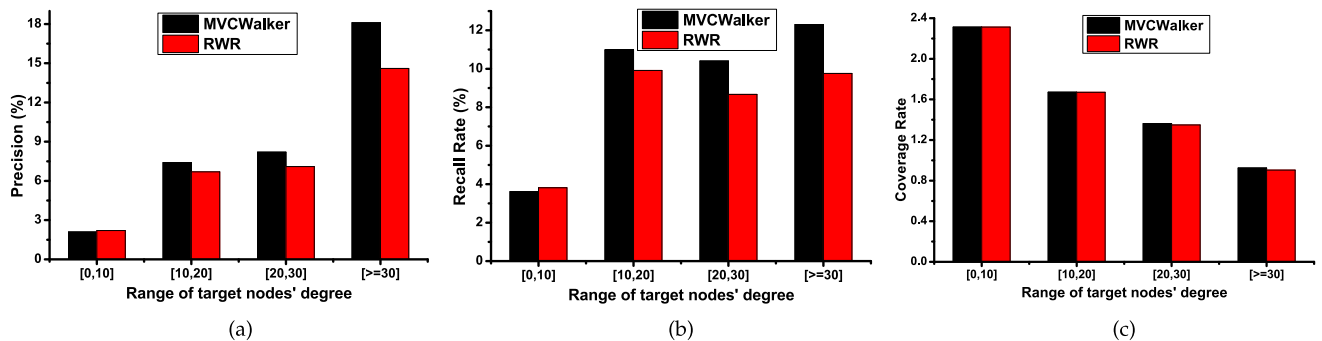
FIGURE 4. Performance of MVCWalker and Basic RWR over Target Nodes' Degree. (a) Precision. (b) Recall Rate. (c) Coverage Rate.
