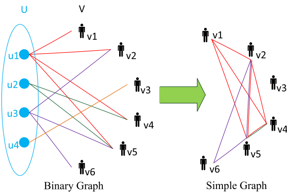
FIGURE 1. Extraction from a Binary Graph to a Simple Graph. U is a list of papers, V is the list of authors. The figure shows three cases: (1) If a scholar has no collaborator, he/she is an isolated node, just like v_3 ; (2) If two authors coauthor a paper, there is a link between them, such as (v_1, v_2) and (v_6, v_5) . (3) If two scholars coauthored multiple papers, the number of links between them increases, like (v_2, v_5) and (v_5, v_4) .
