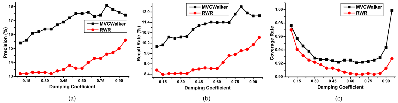
FIGURE 7. Performance of MVCWalker and Basic RWR over Damping Coefficient. (a) Precision. (b) Recall Rate. (c) Coverage Rate.
