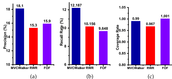
FIGURE 9. Comparison of MVCWalker, RWR and FOF. (a) Precision. (b) Recall Rate. (c) Coverage Rate.
