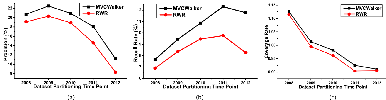
FIGURE 5. Performance of MVCWalker and Basic RWR over Dataset Partitioning Time Point. (a) Precision. (b) Recall Rate. (c) Coverage Rate.
