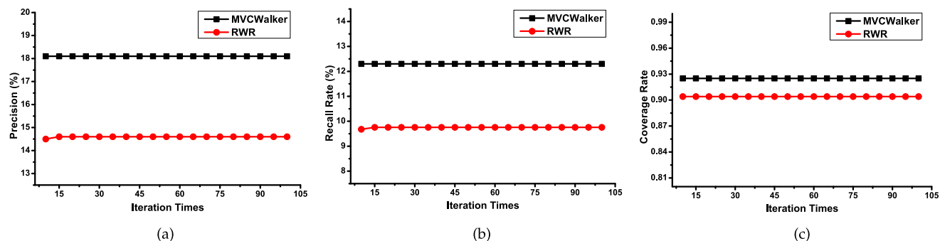
FIGURE 6. Performance of MVCWalker and Basic RWR over Iteration Times. (a) Precision. (b) Recall Rate. (c) Coverage Rate.
