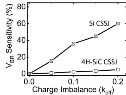
FIGURE 6. Simulated V_{BR} Sensitivity versus charge imbalance of a Si and 4H-SiC CSSJ with N_d = 7 \times 10^{15} \text{ cm}^{-3} , W_n = W_p = 2.5 \mu\text{m} and W_I = 1 \mu\text{m} . For Si CSSJ, data is reproduced from [3].
