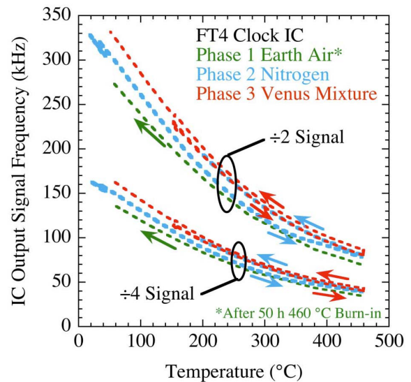
FIGURE 4. Comparison of measured FT4 clock IC signal frequencies as a function of temperature during all three environmental test phases. Arrows indicate where data was taken during temperature ramp-up or ramp-down. For all measurements the IC was powered by V_{DD} = +25 V and V_{SS} = -25 V. The trends shown are consistent with previously reported SiC JFET IC ring oscillator behavior (see text).
