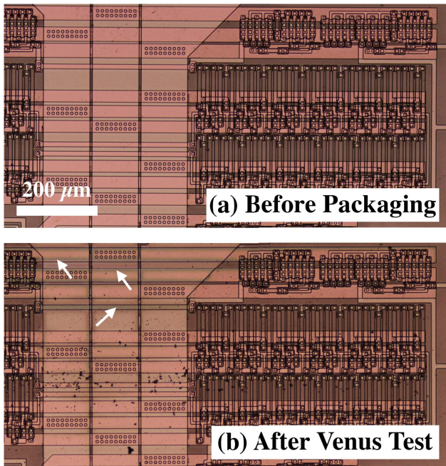
FIGURE 5. Optical micrographs of integrated circuitry on the FT5 \div 2/\div 4 clock IC taken (a) before chip packaging and (b) after completion of the 60-day Venus conditions test. Arrows denote three examples of post-test discoloration in horizontally running Metal 2 traces symptomatic of metal reactions facilitated by cracking of the protective overlying dielectric layers. Dark splotches are particulates on the dielectric-coated chip surface.
